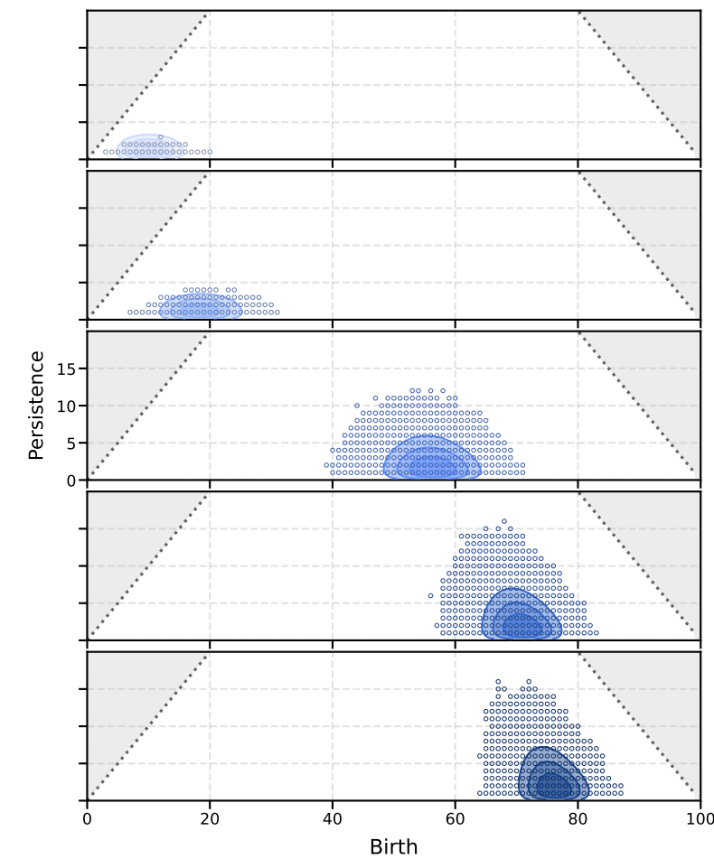
Four-point persistence
