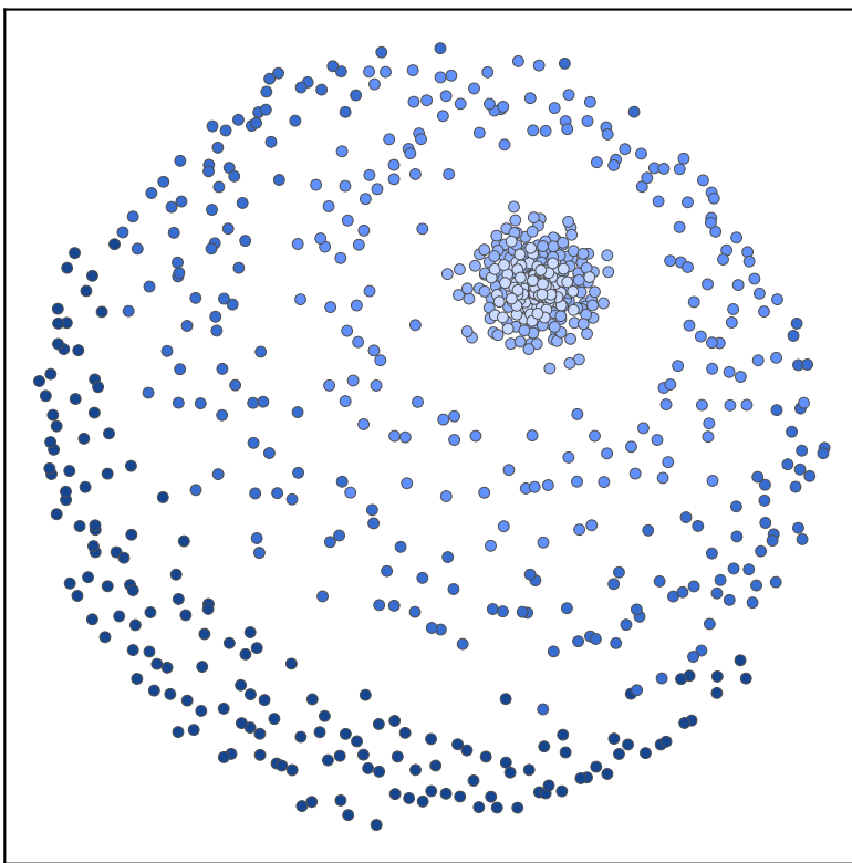
Metric MDS
