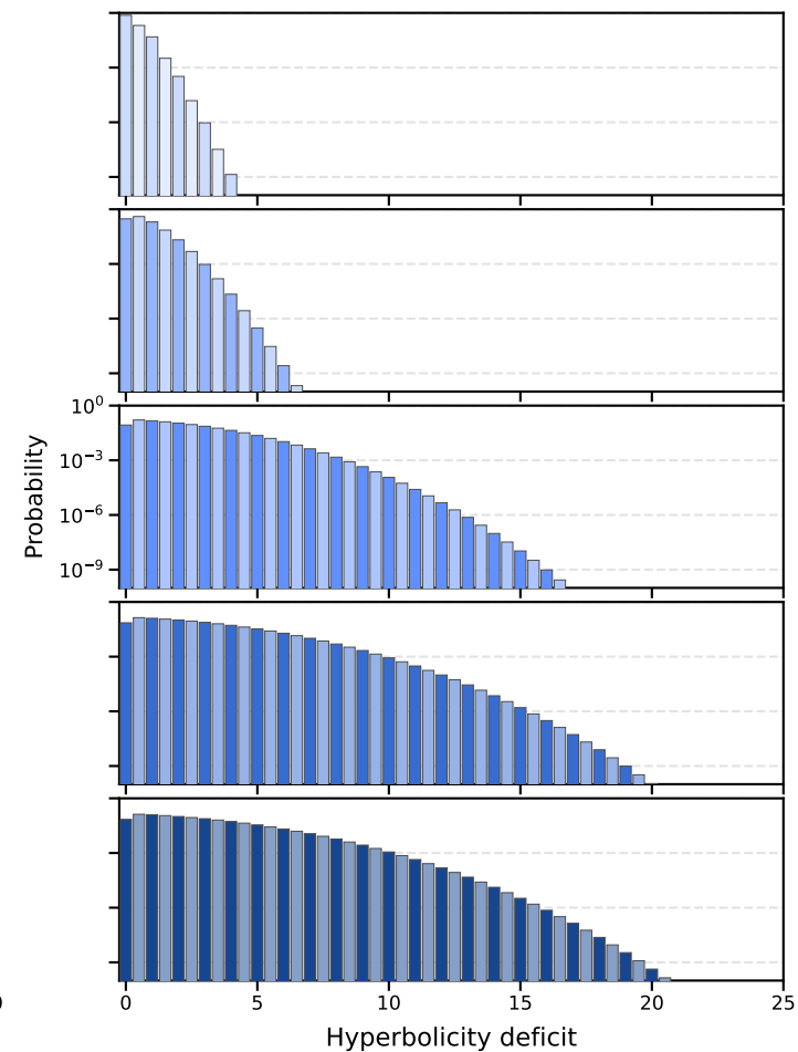
Four-point hyperbolicity
