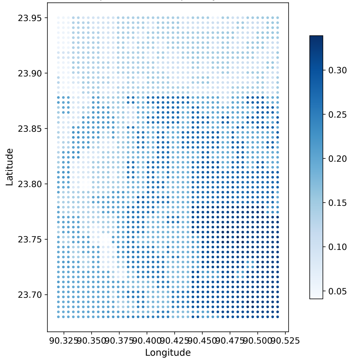
Liquefaction susceptibility index
