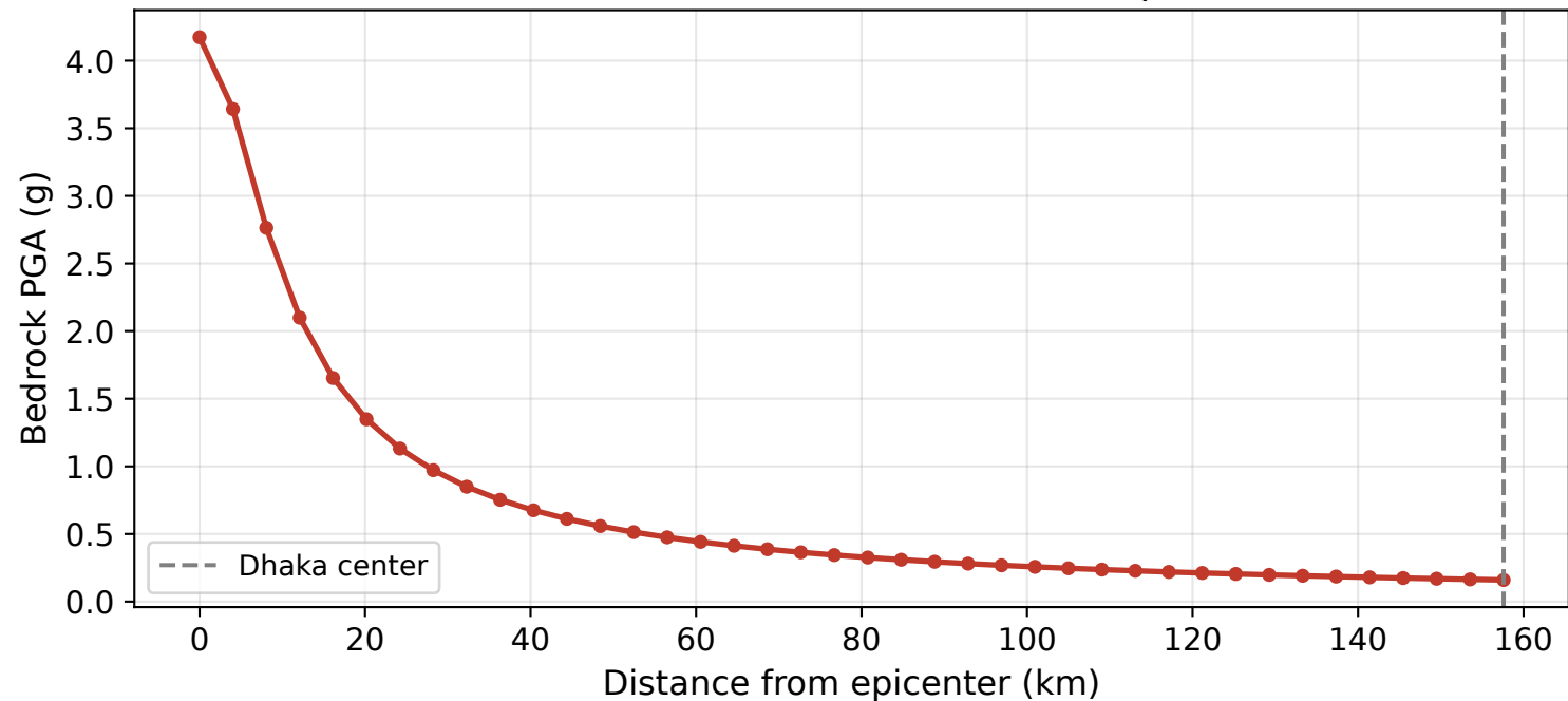
F5.4 — PGA attenuation toward Dauki epicenter
