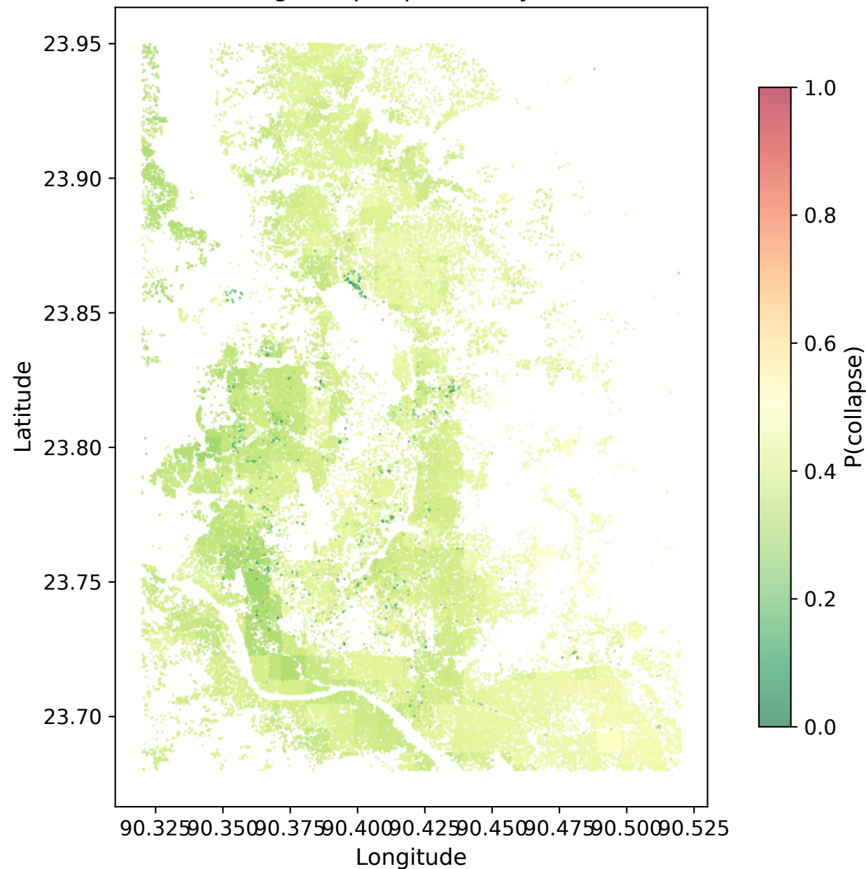
F6.1 — Building collapse probability (Mw 7.2 Dauki)
