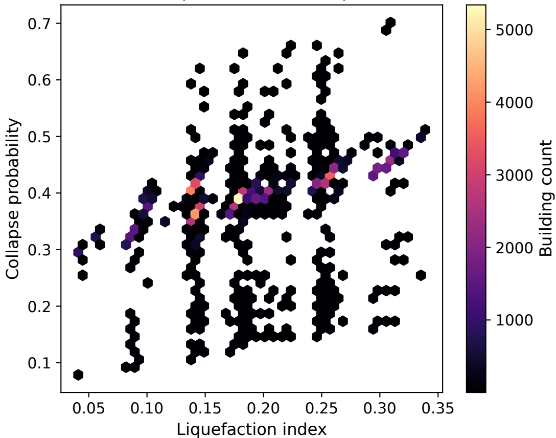
F6.3 — Liquefaction vs collapse risk
