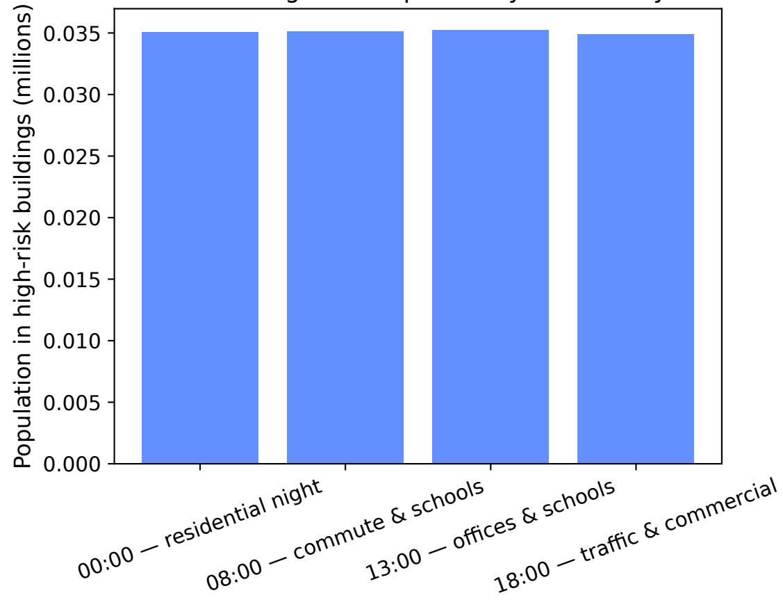
F7.1 — High-risk exposure by time of day
