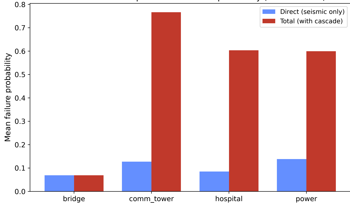
F9.1 — Cascade amplification of failure probability (Mw 7.2 Dauki)
