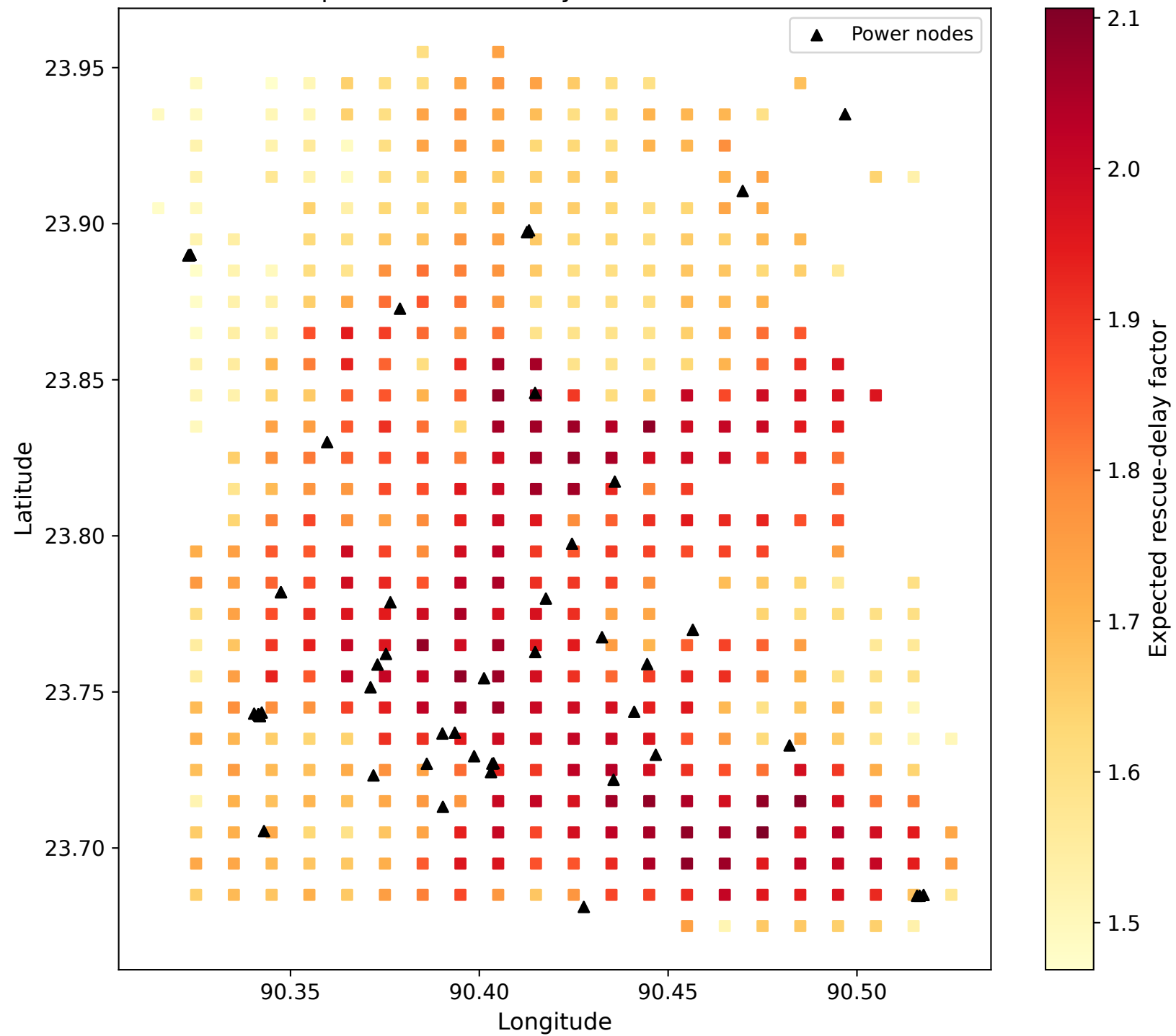
F9.2 — Expected rescue-delay factor from lifeline failures
