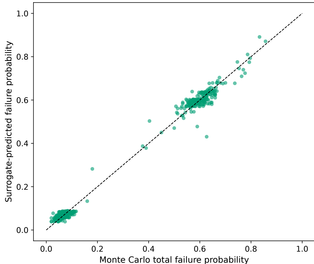
F9.4 — Surrogate emulator vs Monte Carlo (test nodes) GRAPHSAGE MAE = 0.0157, R^2 = 0.9928
