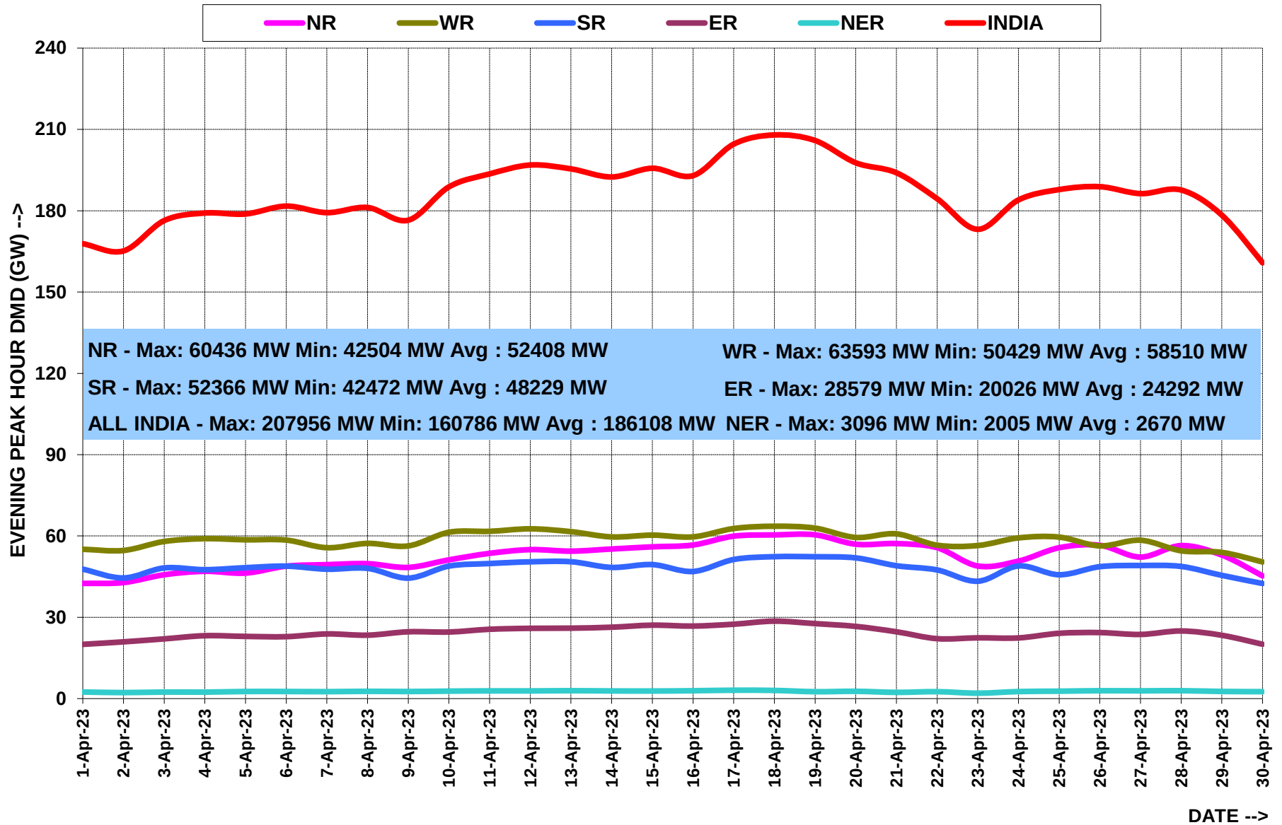
EVENTING PEAK HOUR DEMAND (2000hrs) MET DURING THE MONTH OF APRIL 2023
