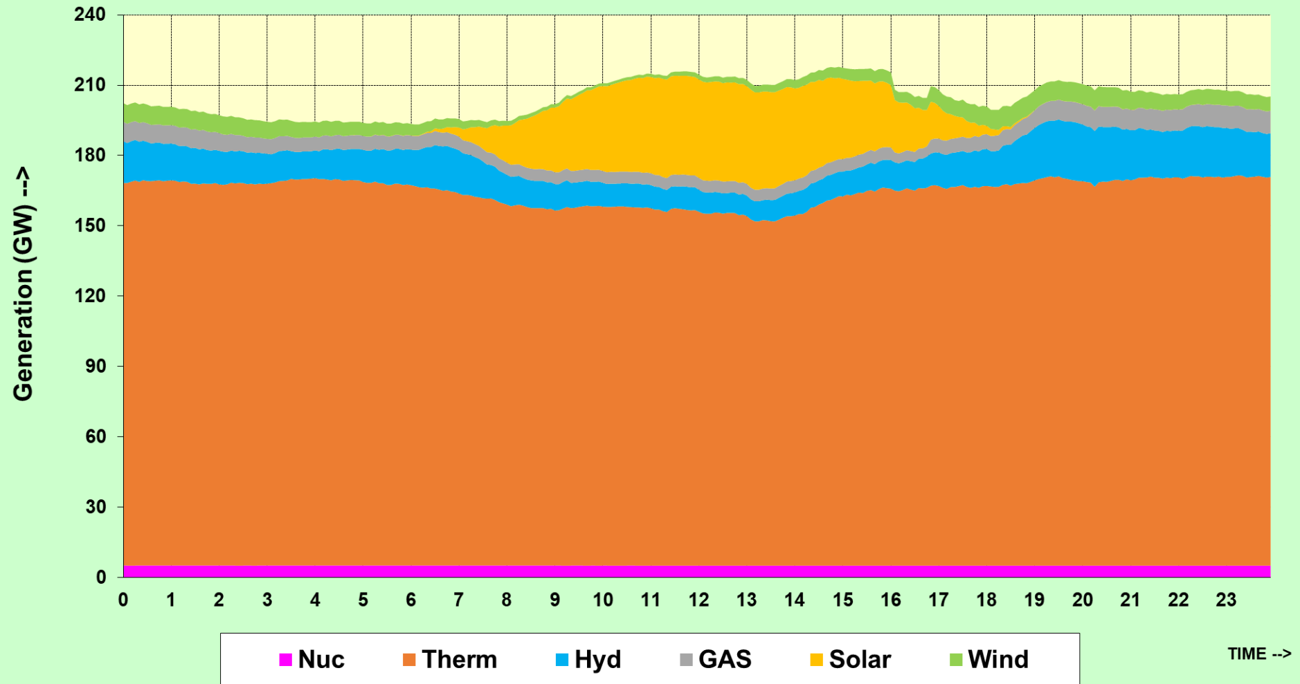
All India Fuel-wise Generation Patterns for 18-APRIL-2023
