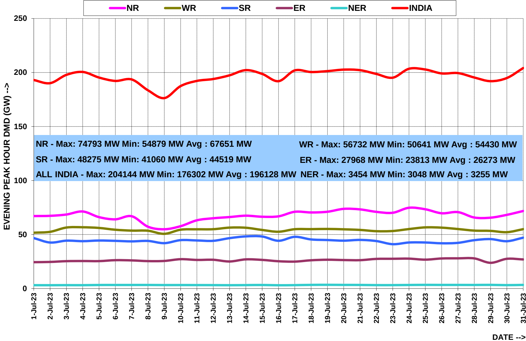
EVENING PEAK HOUR DEMAND(at 2000hrs)MET DURING THE MONTH OF JULY 2023
