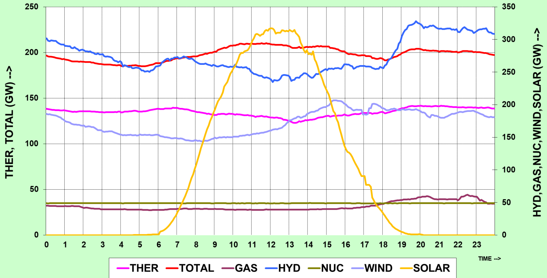
ALL INDIA GENERATION PLOT FOR 21-JULY-2023
