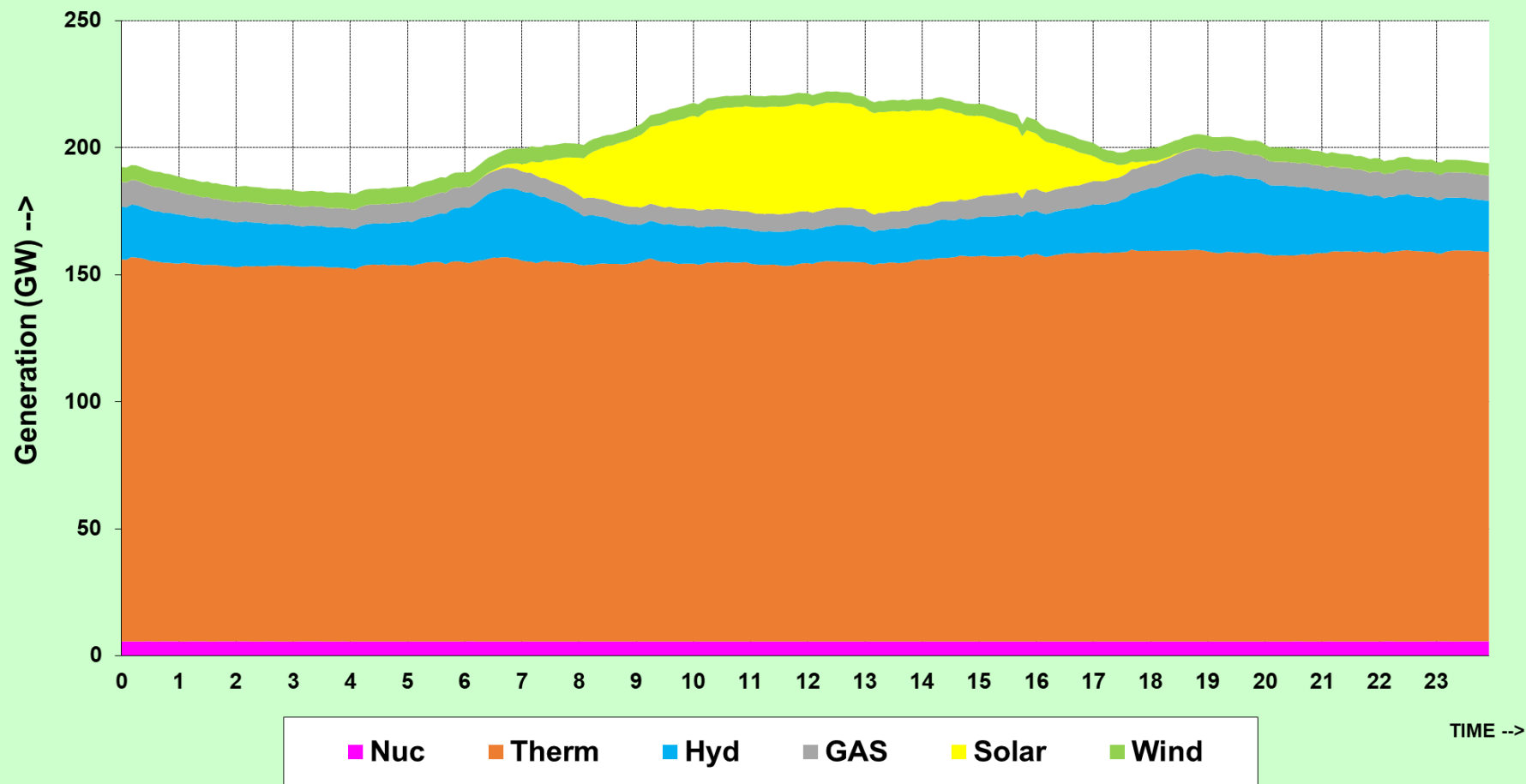
All India Fuel-wise Generation Patterns for 10-OCTOBER-2023
