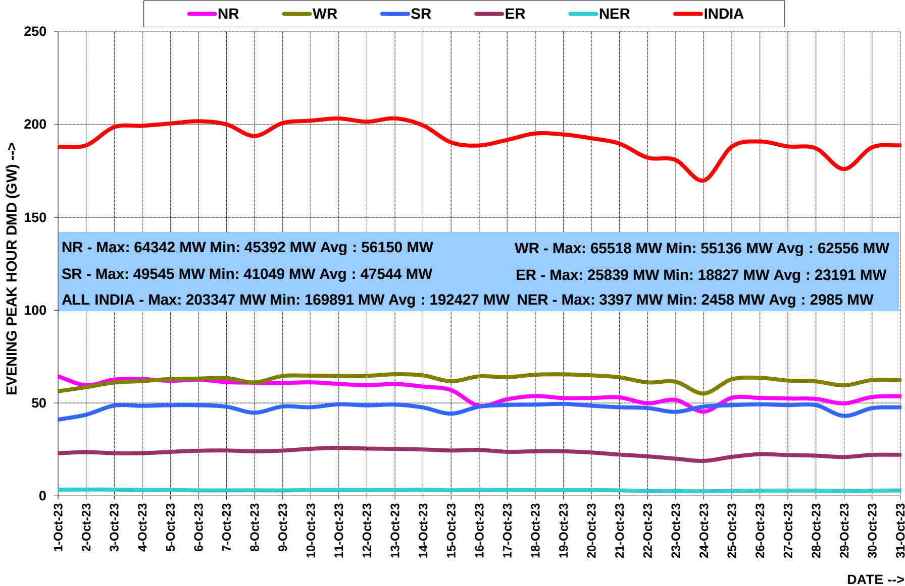
EVENING PEAK HOUR DEMAND(at 1900hrs)MET DURING THE MONTH OF OCTOBER 2023
