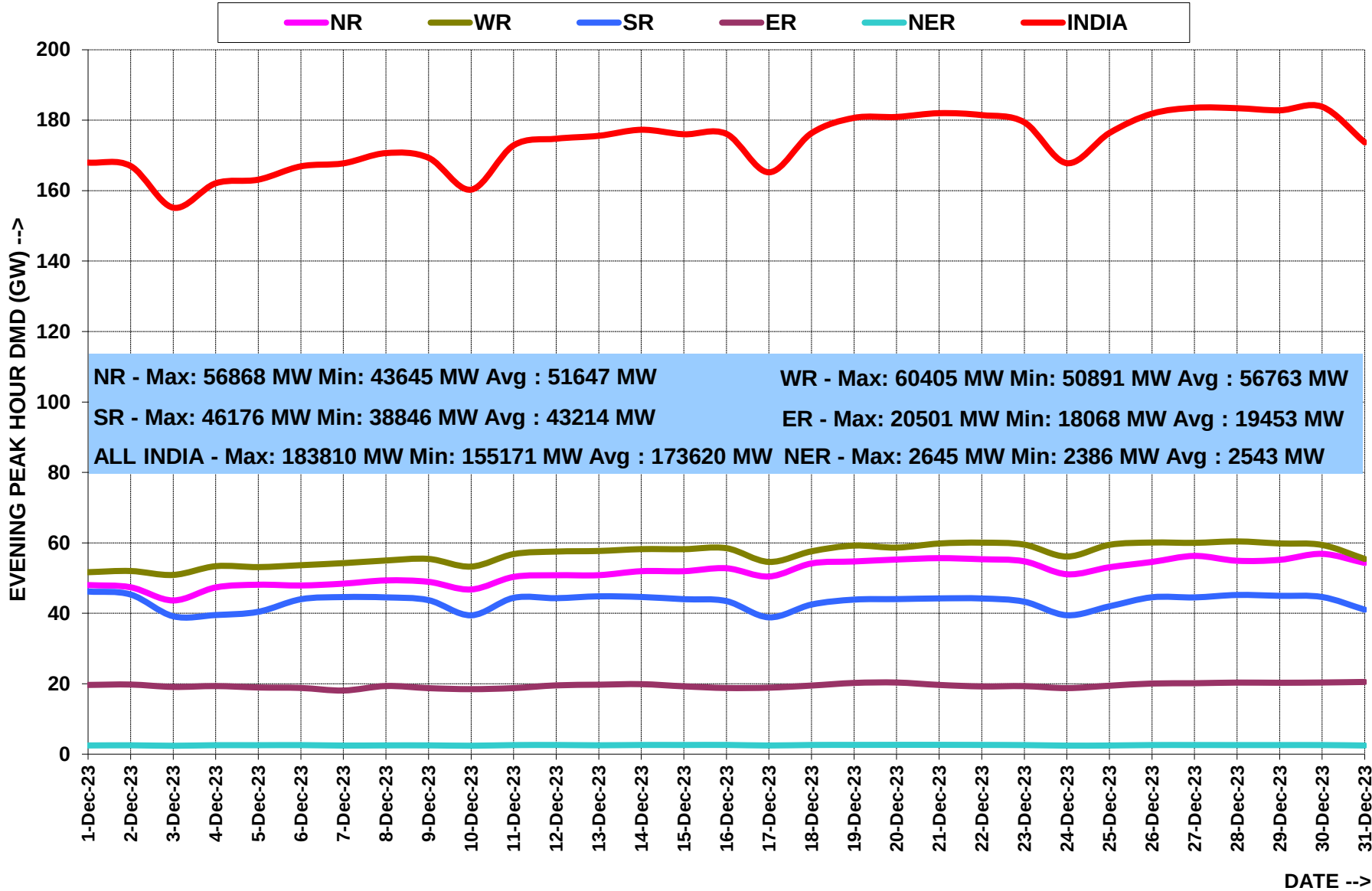
EVENING PEAK HOUR DEMAND(at 1900hrs)MET DURING THE MONTH OF DECEMBER 2023
