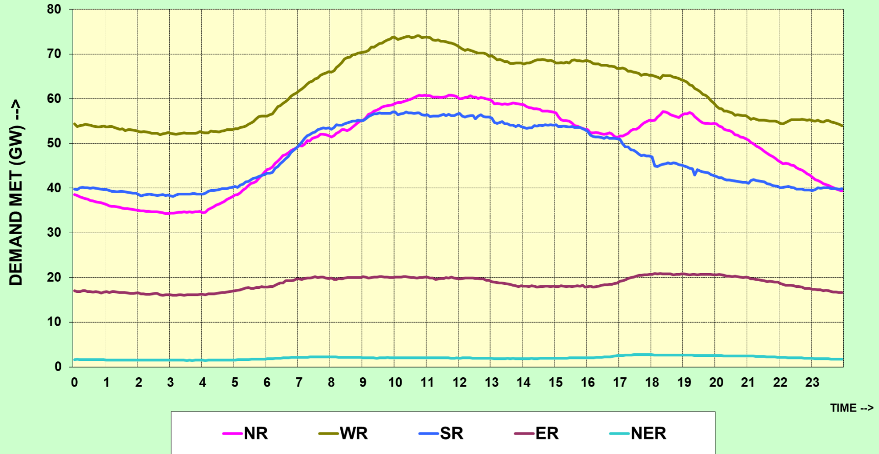
REGIONAL DEMAND MET PLOT FOR 29-DECEMBER-2023
