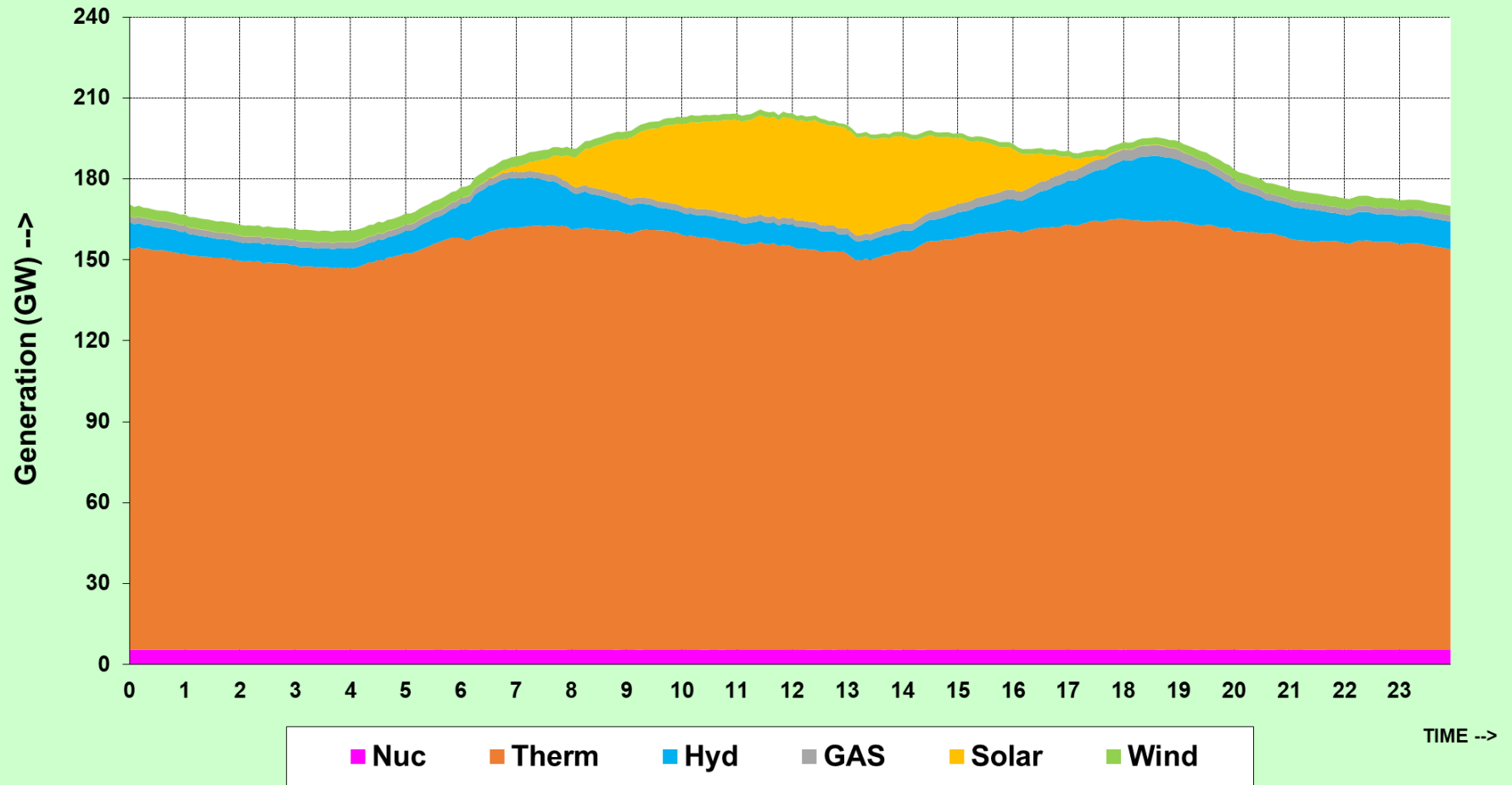
All India Fuel-wise Generation Patterns for 3-NOVEMBER-2023
