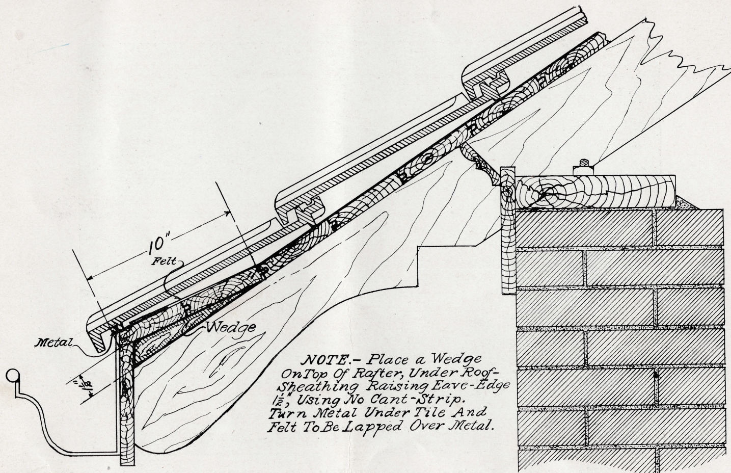
Fig. 86. Detail of Eave Construction.
