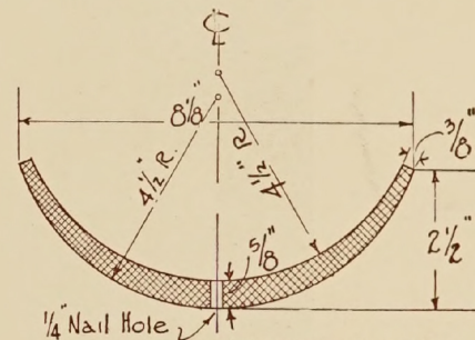
SECTION THRU STANDARD 15" MISSION TILE.
