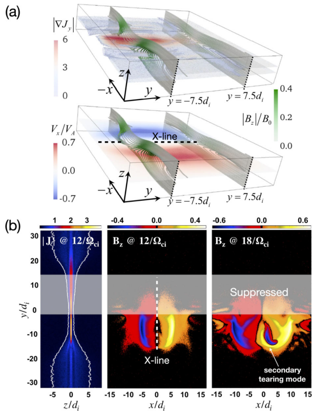
Fig. 9 3D PIC simulation results. (a) 3D view of reconnection with a limited X-line extent, where the thin current sheet region extends 30d_i in y (Huang et al. 2020). The mass ratio in the simulation is 25. (b) The current density on the x = 0 plane (left) and magnetic field B_z on the z = 0 plane (middle and right) (Liu et al. 2019). The mass ratio is 75. The gray shaded area represents the “suppressed reconnecting region”. Adapted from Huang et al. (2020) and Liu et al. (2019)
