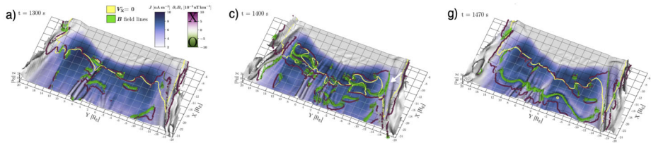
Fig. 19 Evolution of the magnetotail current sheet in a 3D-3V Vlasator simulation. The panels show the current sheet surface (defined as B_r = 0 ) at different times, t = 1300 s (a), t = 1400 s (c), t = 1470 s (g). The color of the surface corresponds to the current density J . The yellow line indicates the flow reversal between the Earthward and tailward reconnection outflow. The magenta and green lines are locations where B_r = 0 and B_z = 0 and correspond to X-lines and O-lines (differentiated using the sign of \partial B_z / \partial r , which is positive at the X-lines and negative at the O-lines). The primary reconnection line is where the X-line (magenta) and flow reversal (yellow) contours are approximately co-located. The background grid shows the coordinates but also the magnetic-field topology: the black grid shows areas where the magnetic field is directed northward, and the white grid shows the areas where it is southward-directed. Adapted from Palmroth et al. (2023)
