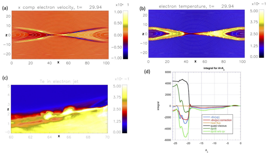
Fig. 7 2D PIC simulation result for magnetotail reconnection. (a) Electron fluid velocity V_{ex} , (b) electron temperature T_e , (c) zoom-in view of T_e , and (d) the heating term in Eq. (65). Adapted from Hesse et al. (2018a, 2019)
