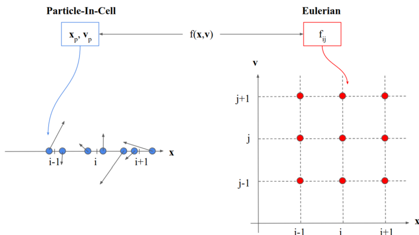
Fig. 16 Sketch of the typical sampling of the plasma distribution function f(\mathbf{x}, \mathbf{v}) adopted in PIC (left) and Eulerian (methods). Adapted from Finelli (2022)
