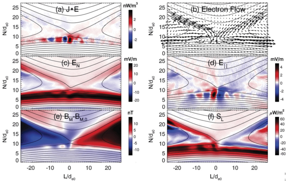
Fig. 8 Simulation results overplotted with magnetic field lines. (a) The \mathbf{J} \cdot \mathbf{E} term from Poynting's theorem; (b) In-plane electron flow field; (c) E_N , the normal component of the electric field; (d) E_{||} , the component of the electric field parallel to the magnetic field; (e) B_M - B_{M,0} , the change in the out-of-plane component of the magnetic field from its (spatially constant) initial value; (f) S_L , the horizontal component of the Poynting flux. Adapted from Swisdak et al. (2018)
