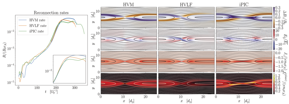
Fig. 17 Magnetic reconnection modeled using three different codes (HVM, HVLF and PIC). Left: normalized reconnection rate R/B_0 v_A . The inset shows the time interval corresponding to the ticker curves in the main plot. To ease the comparison, the curves in the inset are shifted in time. Right: (first row) out-of-reconnection-plane magnetic field \Delta B_z/B_0 = (B_z - B_z(t=0))/B_0 showing the expected Hall quadrupolar pattern; (second row) electric field parallel to the ambient magnetic field E_{\parallel}/E_{\parallel} , where E_{\parallel} is the root mean square of E_{\parallel} in the shown region; (third row) current density in the out-of-plane direction J_z ; (fourth row) electron current density in the plane J_e^{(in-plane)} . The superposed black or white curves are the magnetic field lines. The three columns show results from the three different models. The left column show results from HVM at the simulation time t = 237.5 \Omega_{cp}^{-1} ; the center column show results from the HVLF code at the simulation time t = 232.5 \Omega_{cp}^{-1} ; the right column show results from the PIC code at the simulation time t = 235.0 \Omega_{cp}^{-1} . \Omega_{cp} is the proton cyclotron frequency. Adapted from Finelli et al. (2021)
