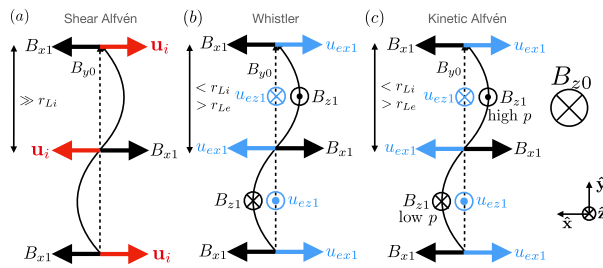
Fig. 2 Sketch of how the Hall effect impacts linear waves in MHD. The wave structure for (a) shear Alfvén waves, (b) parallel propagating whistler waves, and (c) kinetic Alfvén waves. The equilibrium magnetic field B_{y0} is the dashed black arrow. The perturbed magnetic field \mathbf{B}_1 are the black arrows. The perturbed ion bulk flow \mathbf{u}_i are the red arrows, which occur in (a) because the wavelength is much larger than the ion gyroradius. In (b) and (c), the wavelength is at or below ion gyroscscales, so the bulk flow is due to electron motion in the blue arrows. In (c), there is a large out-of-plane equilibrium magnetic field B_{z0} , so the magnetic perturbation B_{z1} changes the magnetic pressure which to first order and requires a change to the gas pressure p
