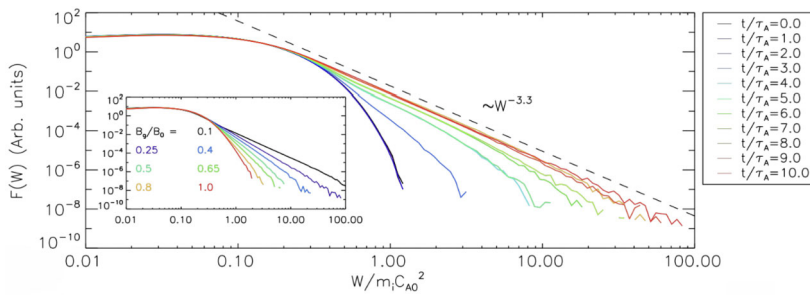
Fig. 15 Energetic electron spectra from kglobal . A log-log plot of the electron differential density F(W) versus energy ( W ) at multiple times from a reconnection simulation with a guide field B_g/B_0 = 0.25 . A power-law develops after t/\tau_A \sim 3 - 5 . Inset: The late-time F(W) for several guide fields, illustrating the dependence on the ratio of the guide-to-ambient magnetic field. Adapted from Arnold et al. (2021)
