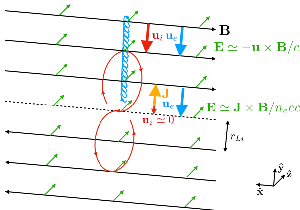
Fig. 1 Physics of the Hall effect in reversing magnetic fields. A reversing anti-parallel magnetic field in the \pm \hat{x} direction is drawn using black arrows, with the neutral line as the dashed line. A uniform electric field in the \hat{z} direction is drawn in green. The smaller blue trajectory is that of an electron E \times B drifting towards the neutral line with bulk velocity \mathbf{u}_e . An ion E \times B drifting far from the neutral line has bulk ion velocity \mathbf{u}_i identical to \mathbf{u}_e , so the electric field in this region is given by \mathbf{E} = -\mathbf{u} \times \mathbf{B}/c , where \mathbf{u} is the single fluid (MHD) bulk flow velocity. Within an ion gyroradius r_{Li} of the neutral line, the electron continues with bulk flow \mathbf{u}_e , while the ion demagnetizes (in the red trajectory) and \mathbf{u}_i becomes small. In this region, there is a non-zero current density \mathbf{J} (orange), and the electric field in this region is predominantly given by the Hall electric field \mathbf{E} = \mathbf{J} \times \mathbf{B}/n_e e c
