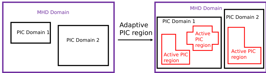
Fig. 13 A schematic shows the improvement of the MHD-AEPIC (right) model from the MHD-EPIC (left) model. Adapted from Chen et al. (2023)
