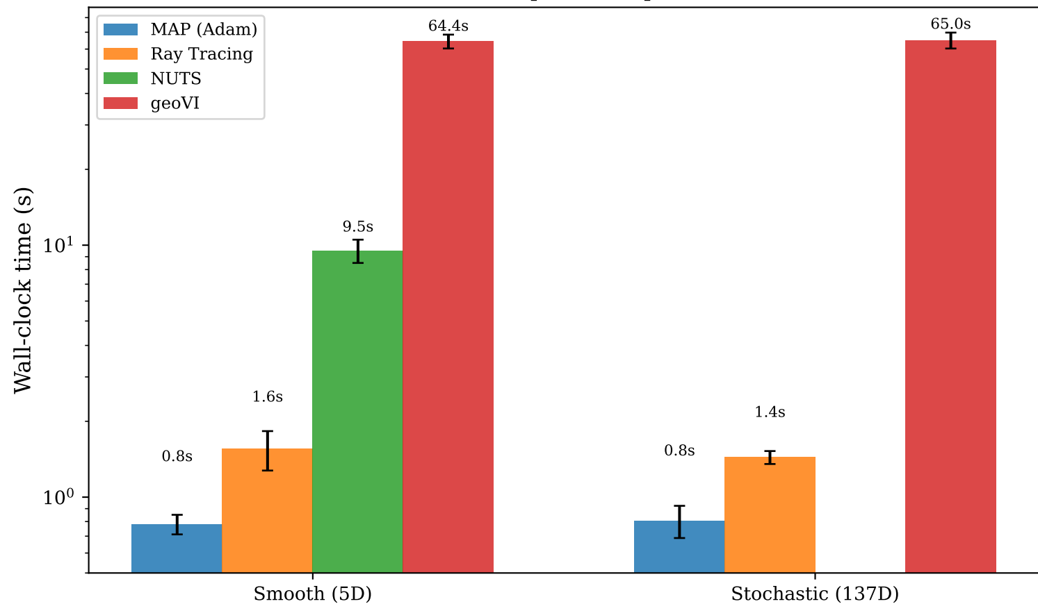
Inference Speed Comparison
