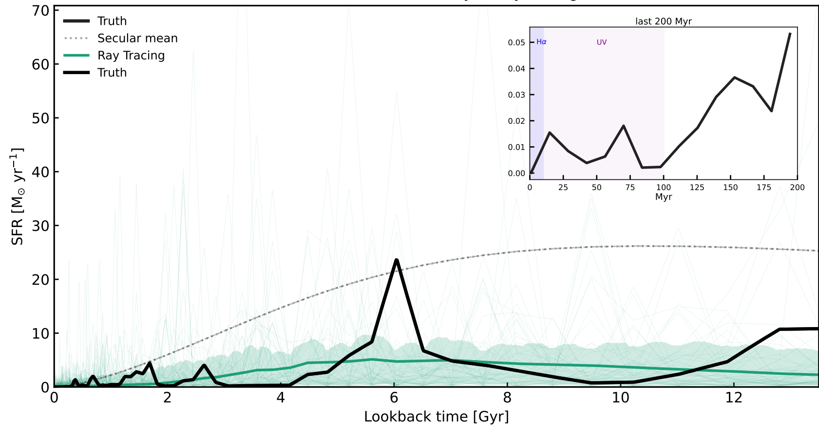
Stochastic SFH Recovery — Ray Tracing
