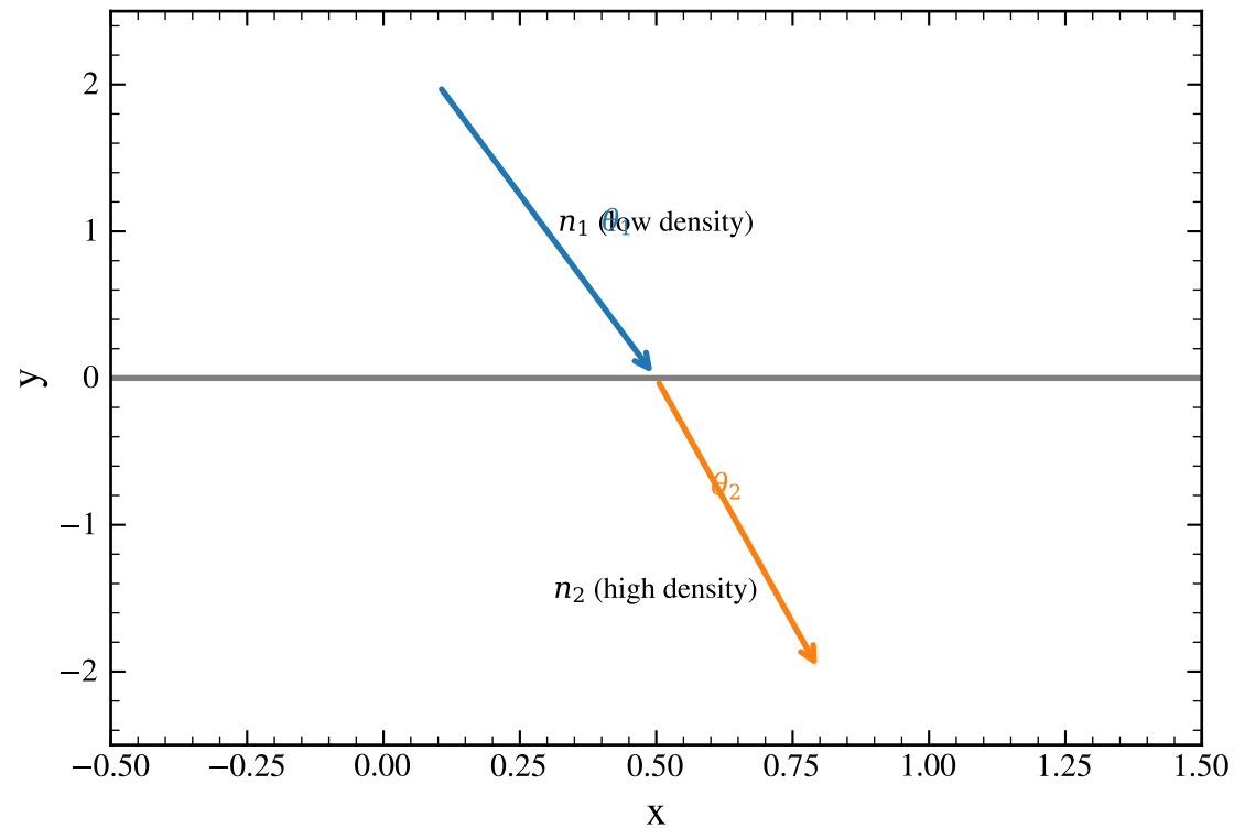
Classical Snell's Law
