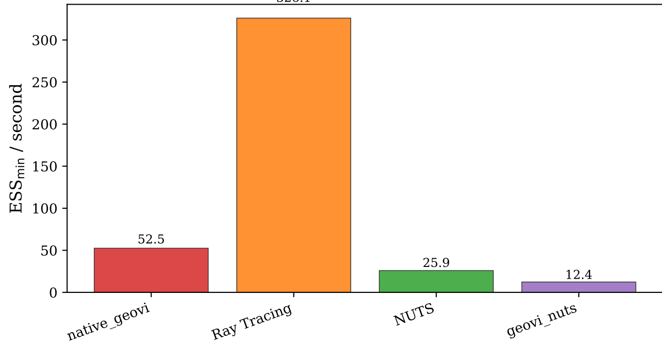
Inference Efficiency: ESS per Second (D=7 Smooth)
