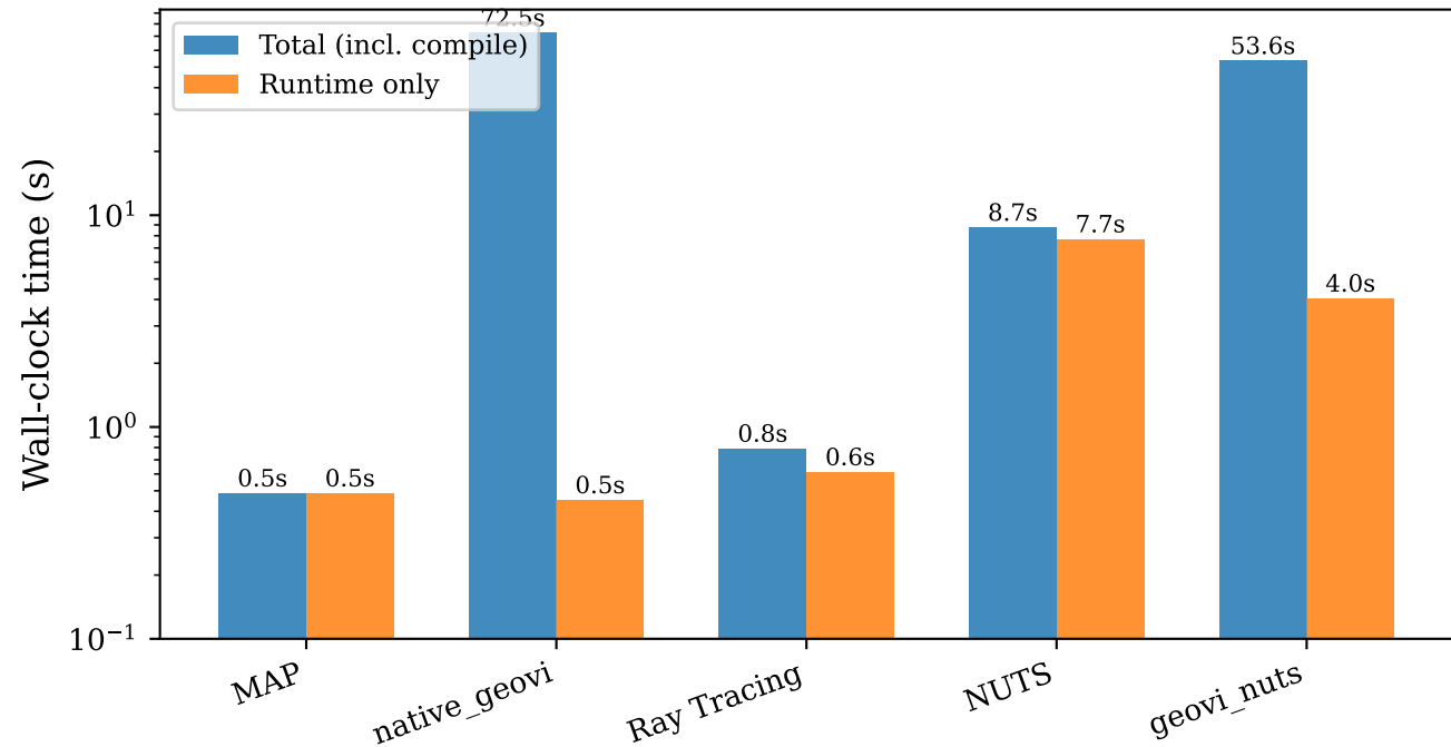
Inference Wall-Clock Time (D=7 Smooth)
