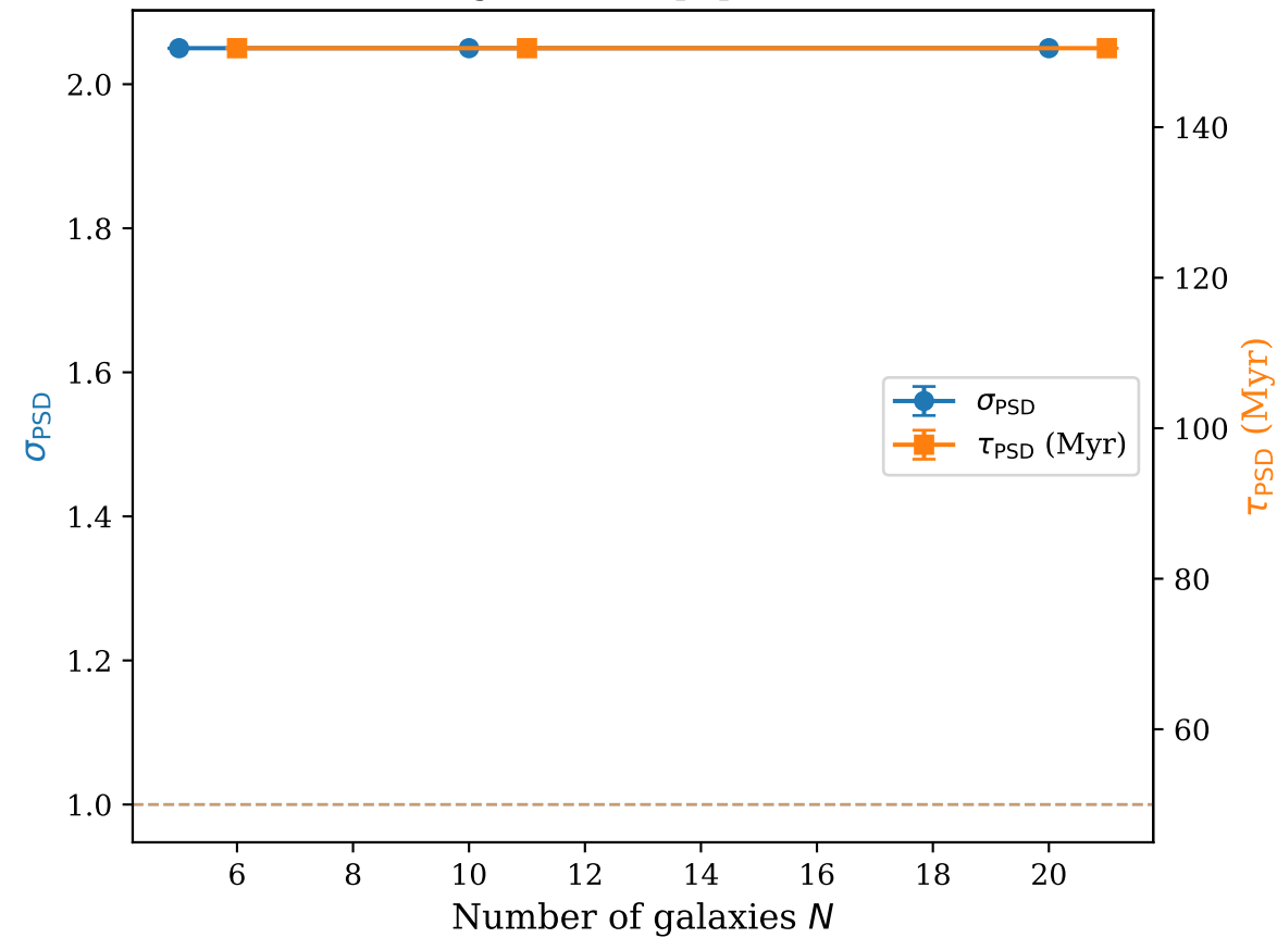
Convergence with population size
