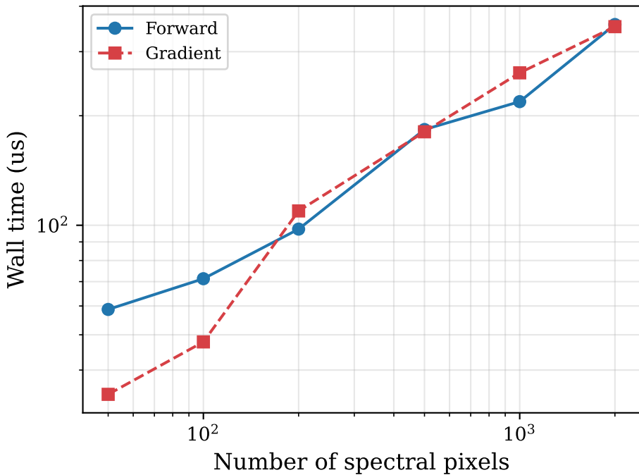
Scaling: Number of spectral pixels
