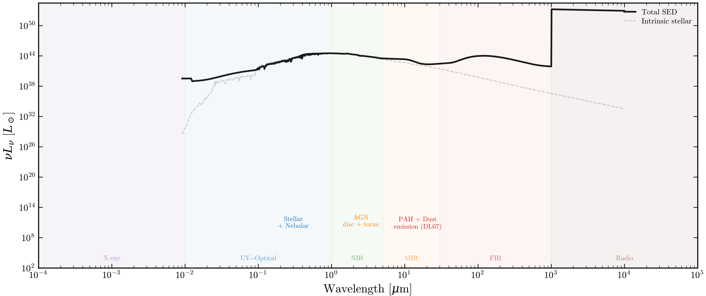
diffsed panchromatic wavelength coverage: X-ray to radio
