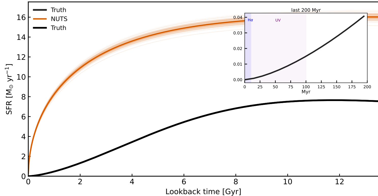
SFH Recovery — Parametric (NUTS)
