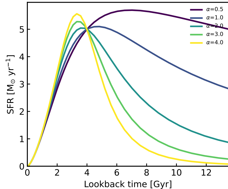
Vary \alpha (right side: early universe)
