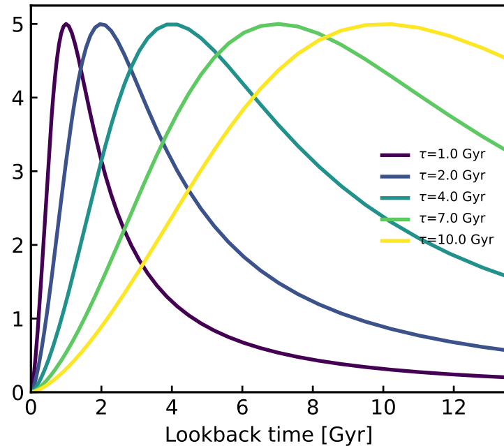
Vary \tau (peak lookback time)
