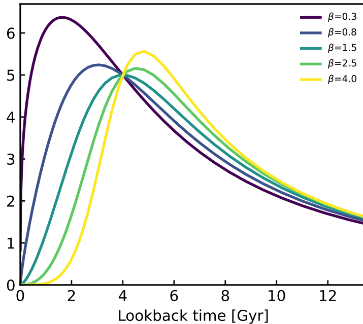
Vary \beta (left side: near present)
