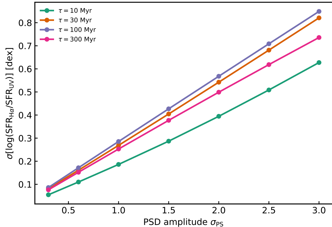
\text{H}\alpha/\text{UV} ratio scatter vs. PSD amplitude
