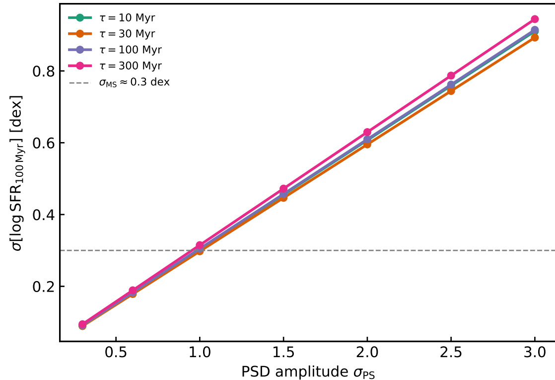
SFR scatter vs. PSD amplitude
