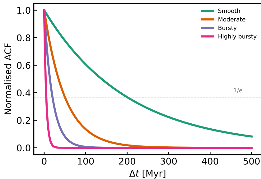
Autocorrelation
