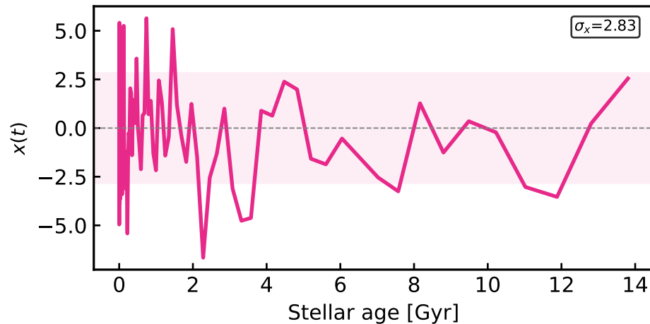
Highly bursty: \sigma_{\text{PS}}=4.0 , \tau_{\text{PS}}=5 Myr
