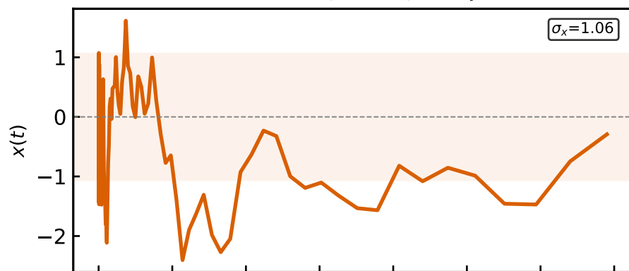
Moderate: \sigma_{\text{PS}}=1.5 , \tau_{\text{PS}}=50 Myr
