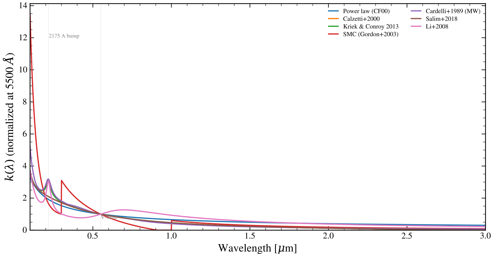
Dust Attenuation Curves in diffsd
