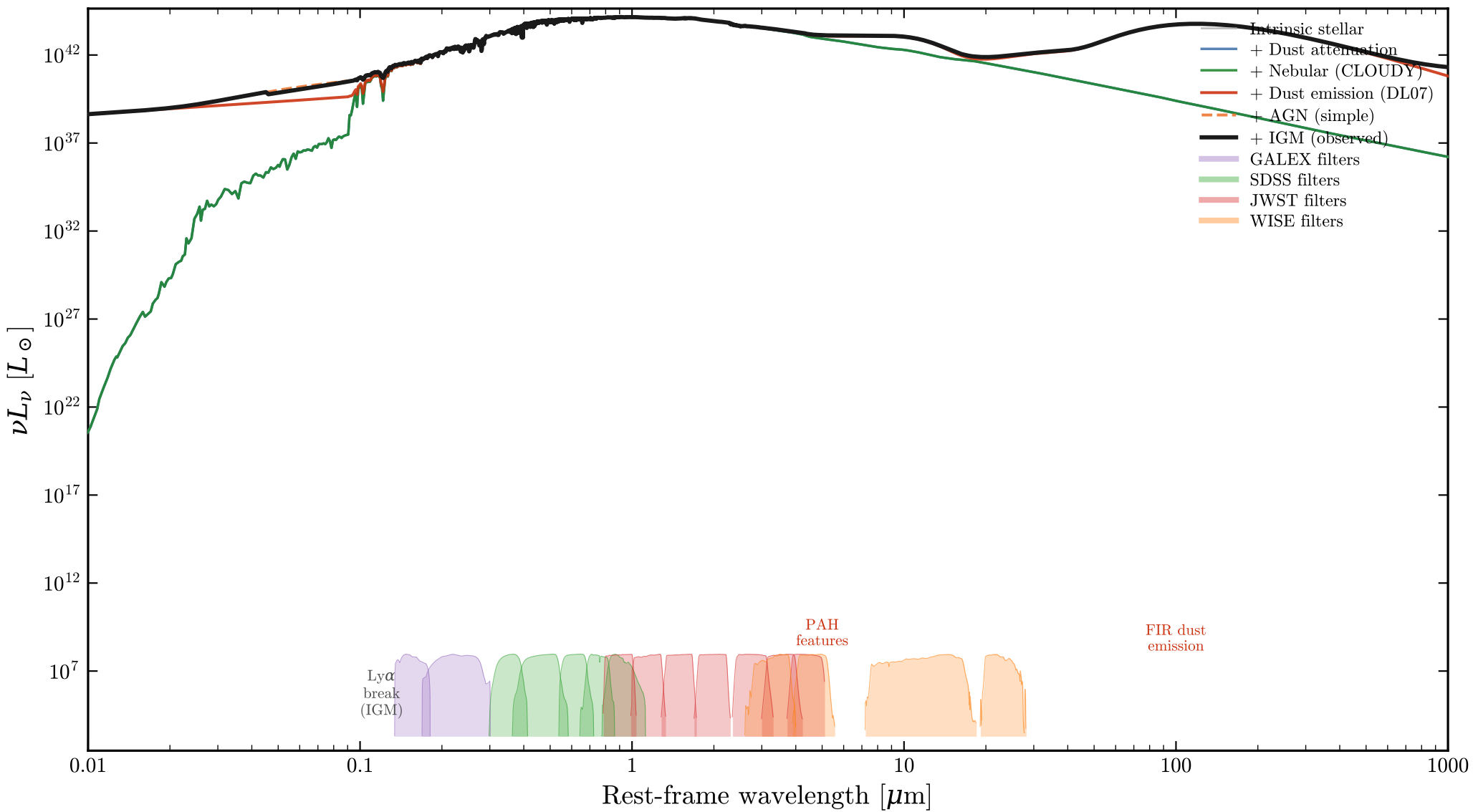
diffsed forward model: star-forming galaxy at z = 1
