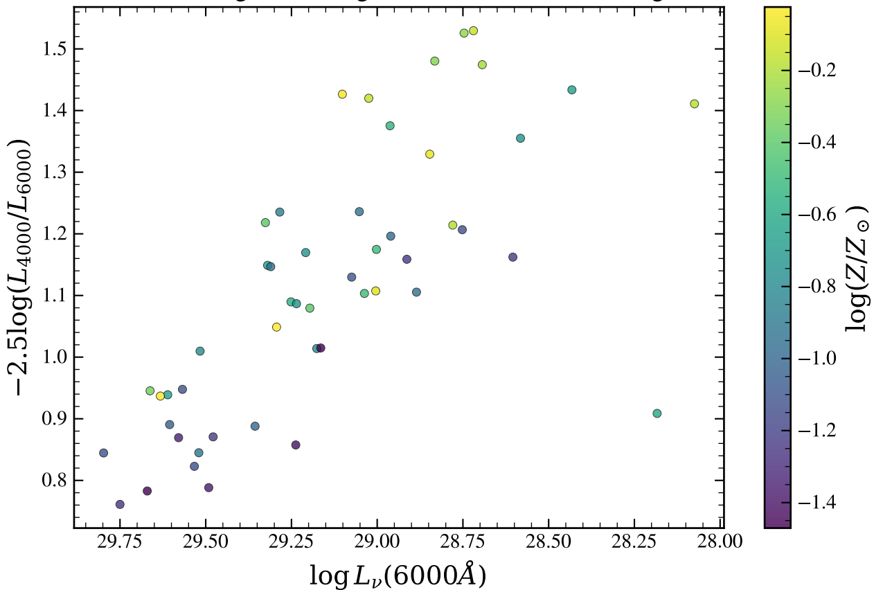
Color-Magnitude Diagram from Simulated Catalog
