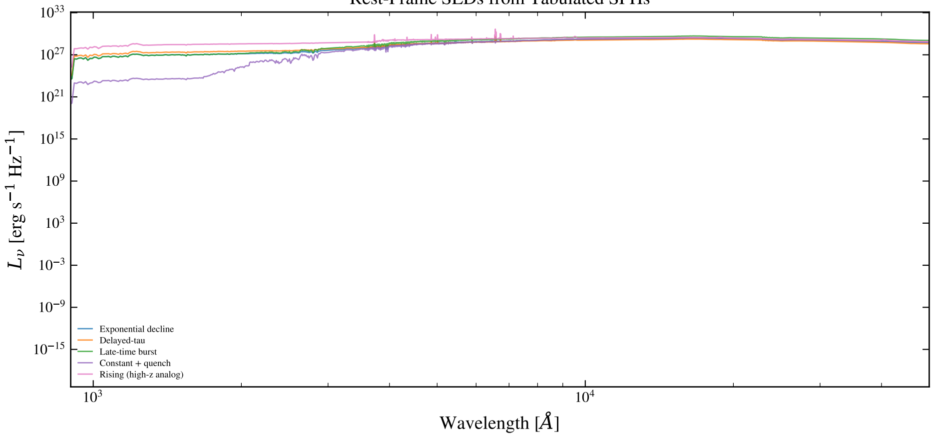
Rest-Frame SEDs from Tabulated SFHs
