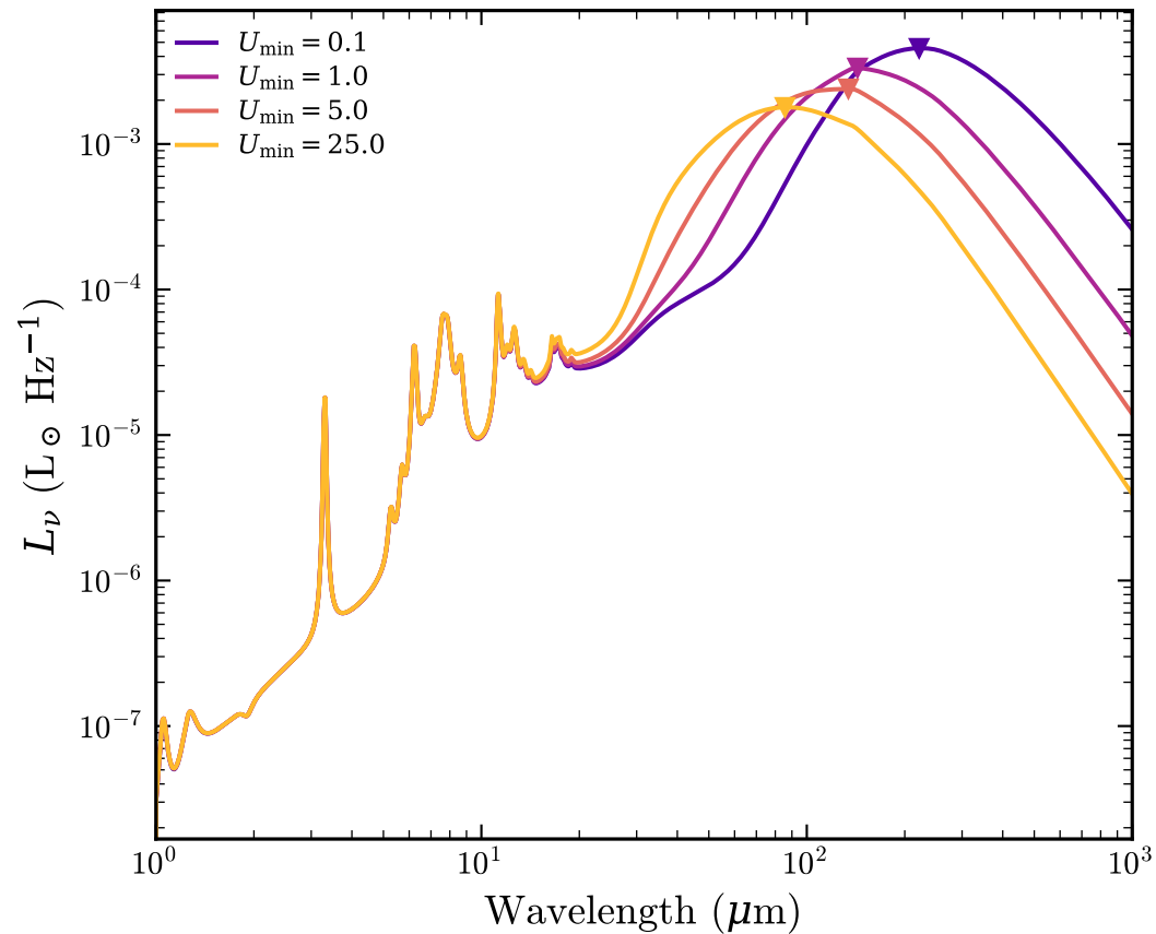
DL07 tabulated: varying U_{\min}
