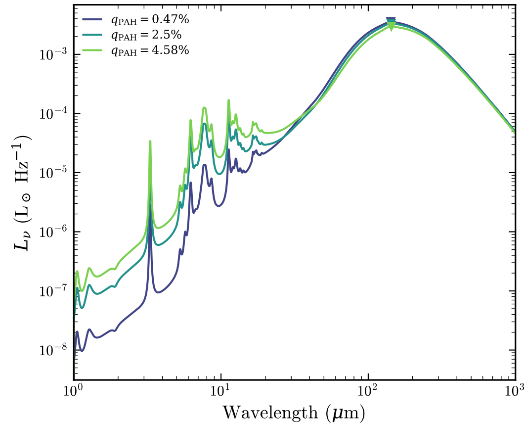
DL07 tabulated: varying q_{\text{PAH}}
