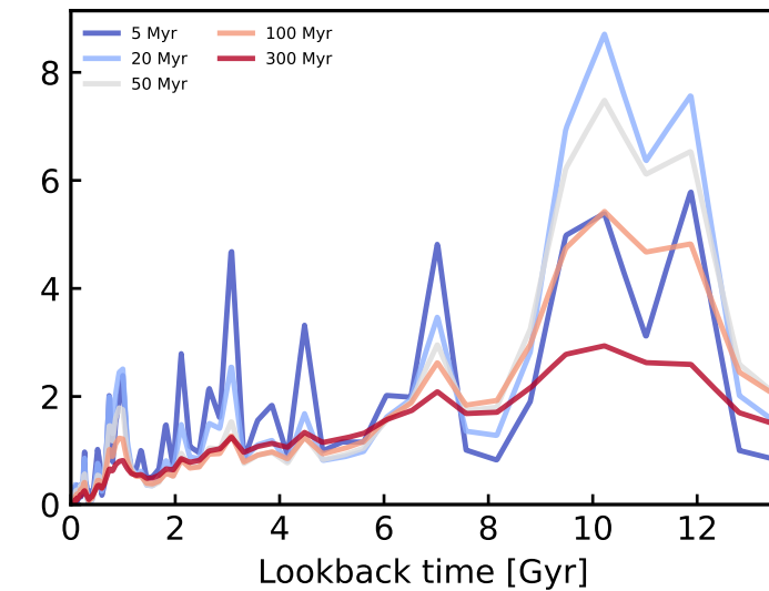
Vary \tau_{\text{PS}}
