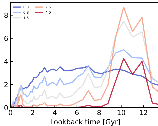
Vary \sigma_{\text{PS}}
