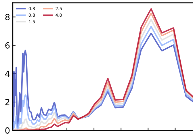
Vary \beta
