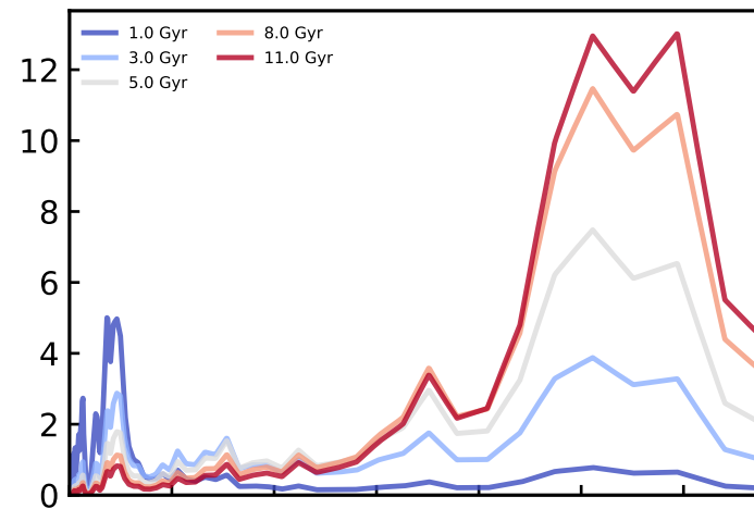
Vary \tau_{\text{mean}}
