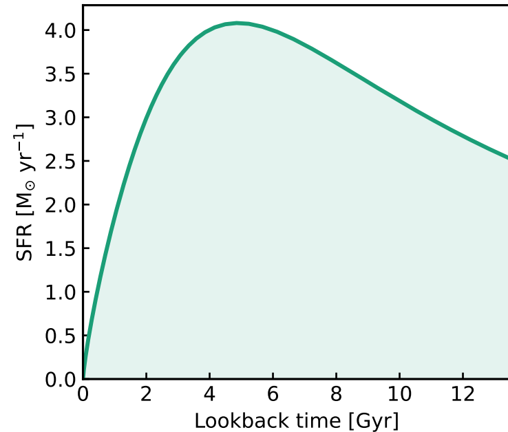
Step 1: Secular mean \overline{\text{SFR}}(t)
