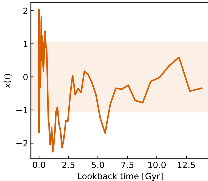
Step 2: GP field ( \sigma_{\text{PS}}=1.5 , \tau_{\text{PS}}=50 Myr)
