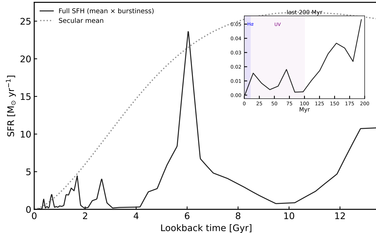
True Bursty SFH ( \sigma_{\text{PS}} = 2.0 , \tau_{\text{PS}} = 20 Myr)
