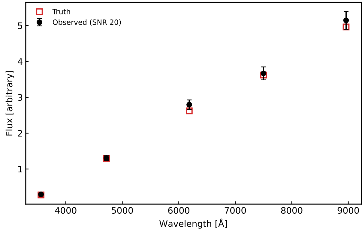
Mock SDSS Photometry — Stochastic SFH
