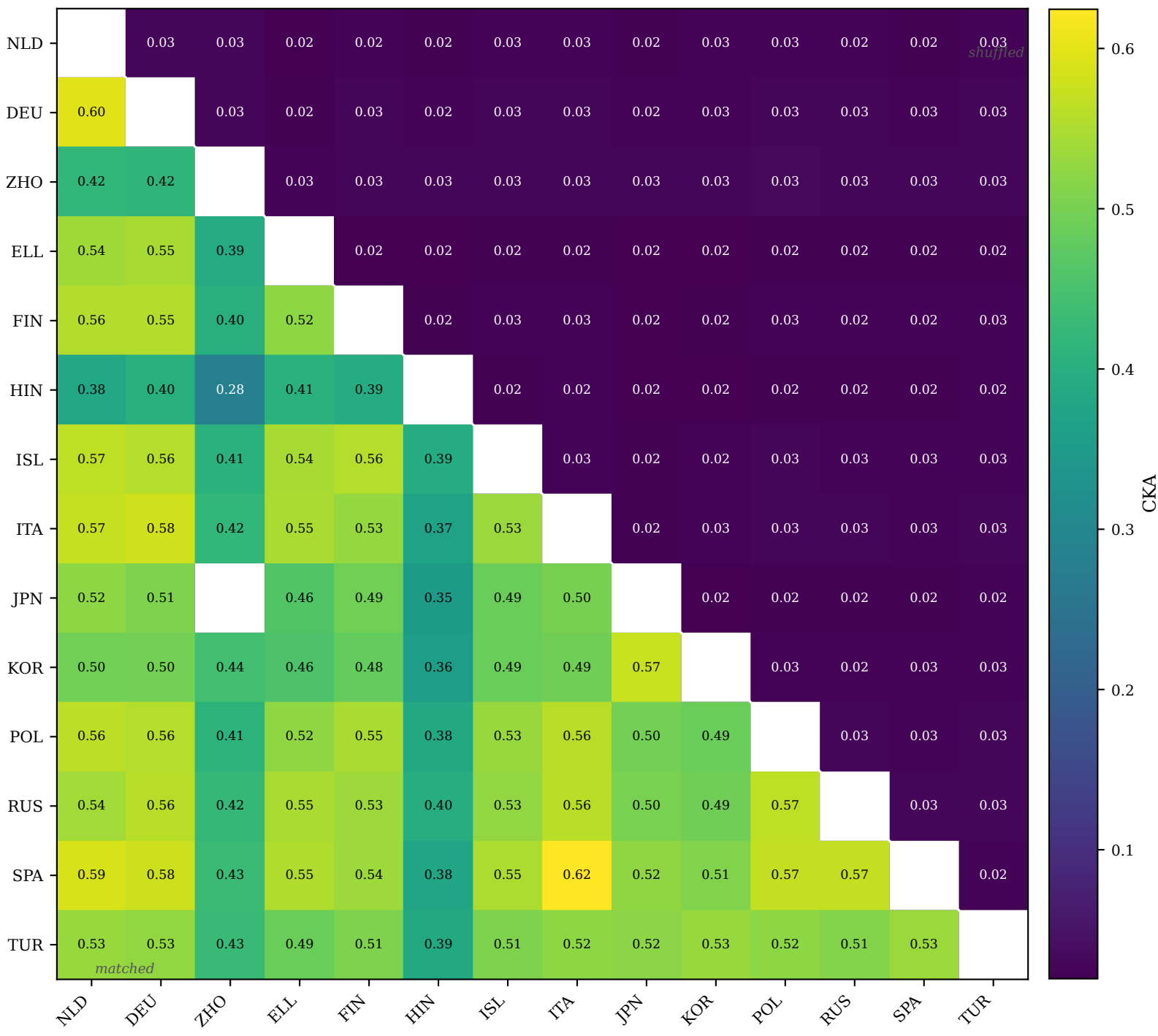
Final-layer CKA (Sentence SGPT-weighted Pooling, main)
