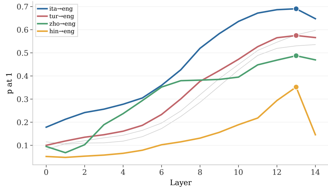
All 6 directed pairs (dot = that pair's best layer)
