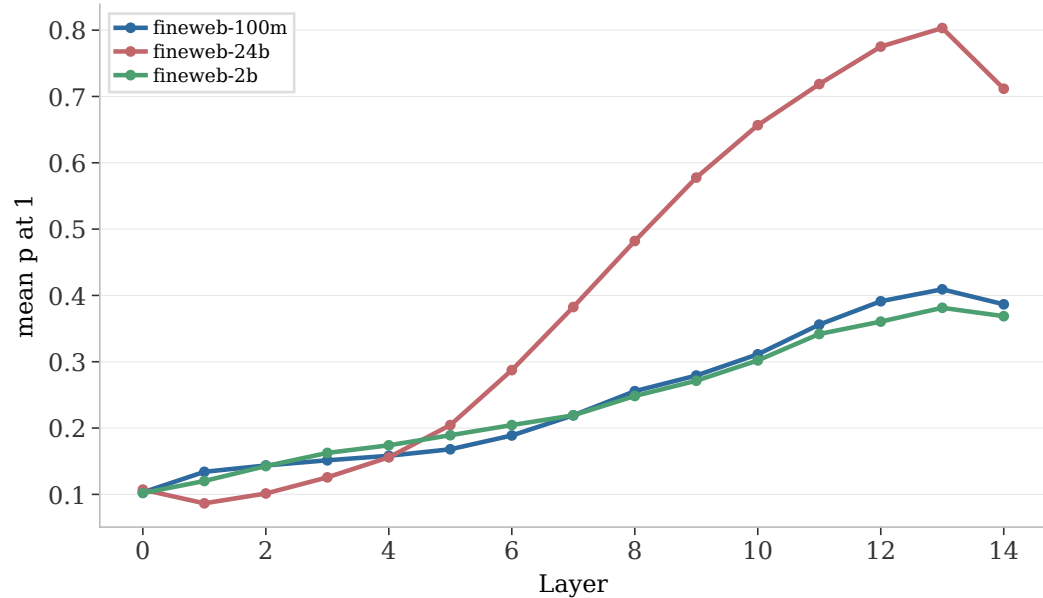
Mean by layer, grouped by scale
