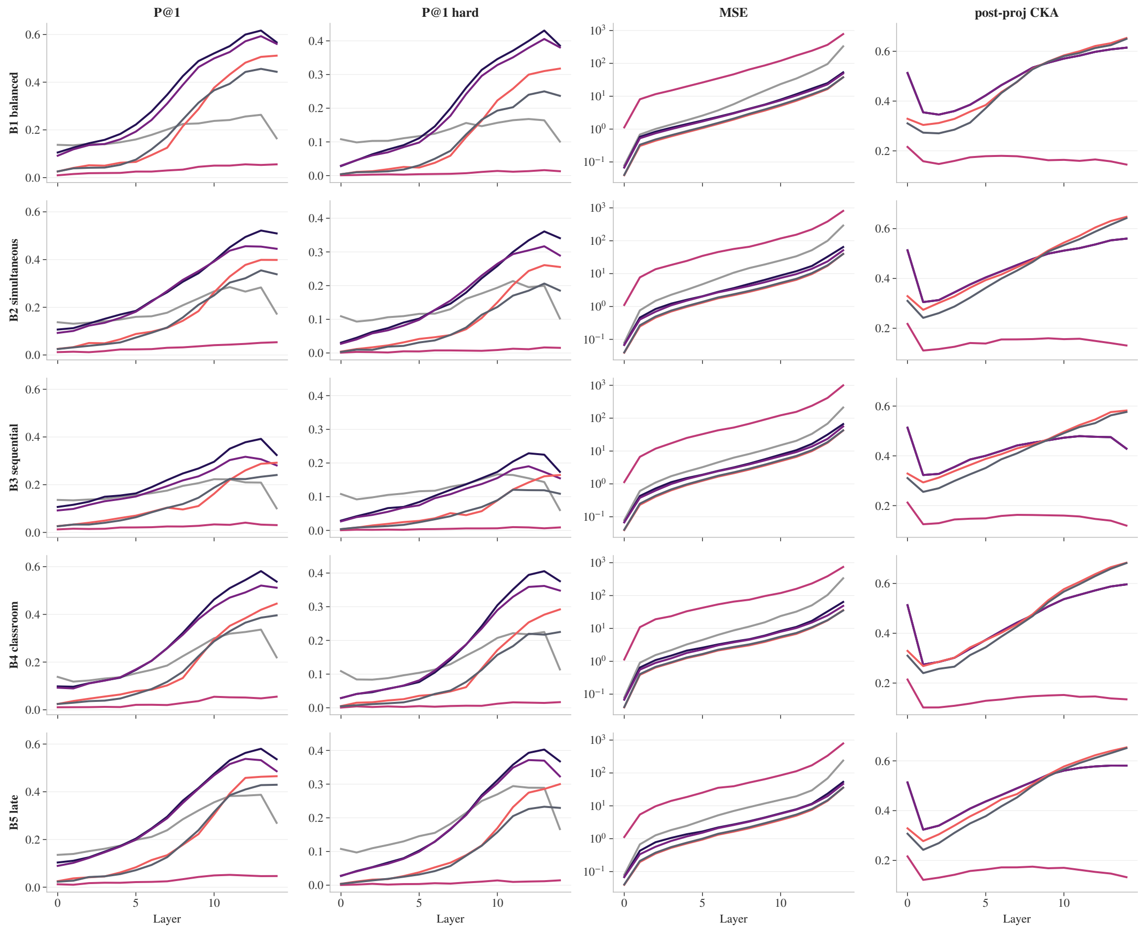
Reconstruction method \times metric \times layer — curricula (c)
