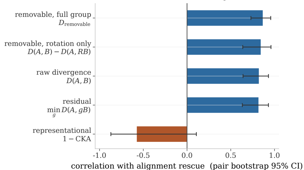
(b) which notion of “different” predicts it
