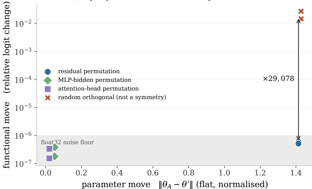
(a) equal parameter movement, unequal functional cost
