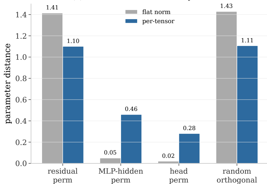
(b) the flat norm reorders the symmetries
