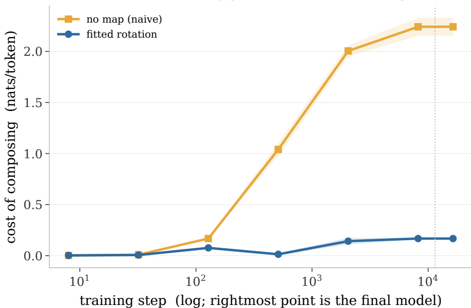
(a) incompatibility grows 1000 \times across training
