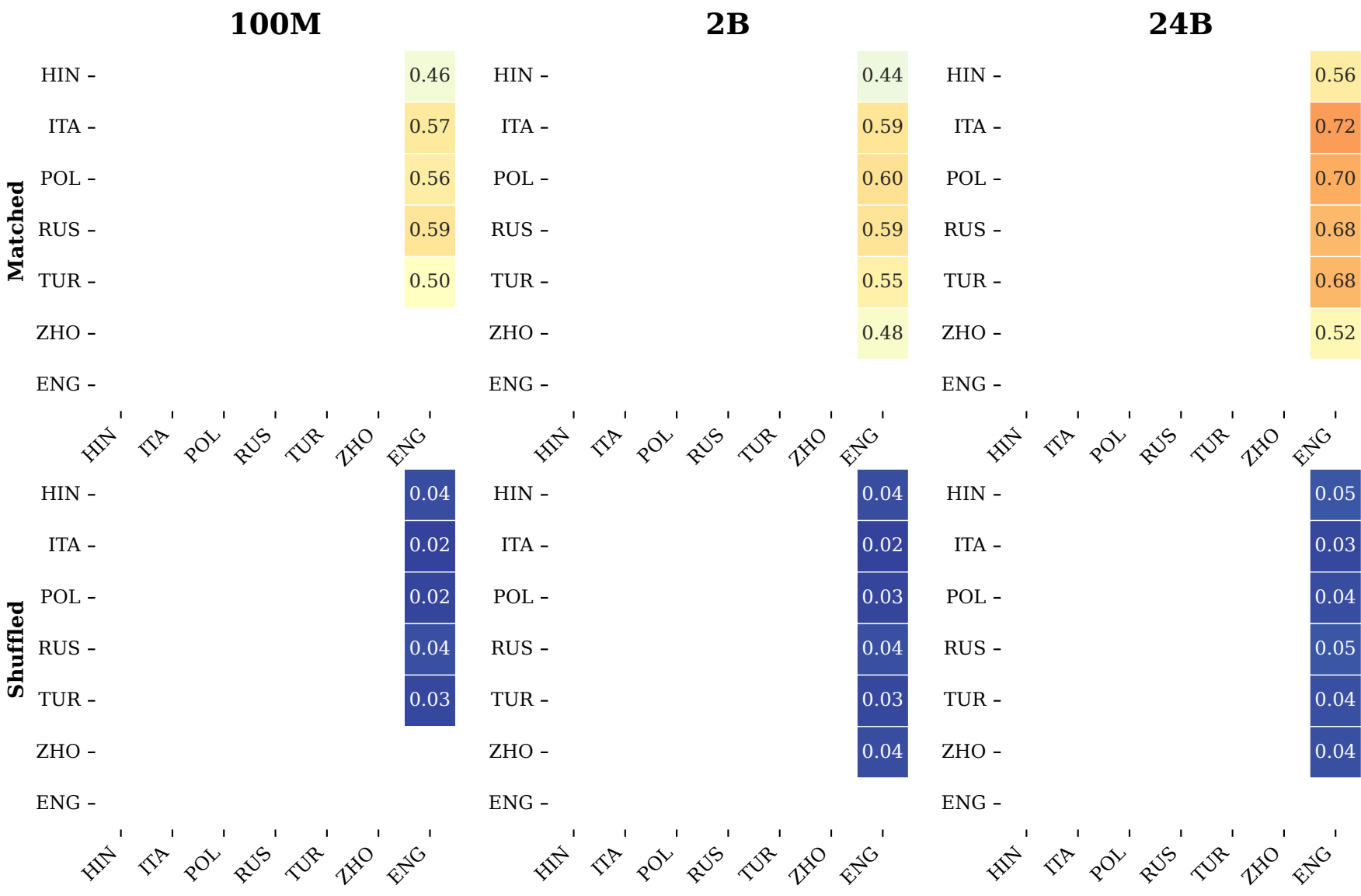
Last-layer pairwise CKA across data scale (Beetle bilingual)
