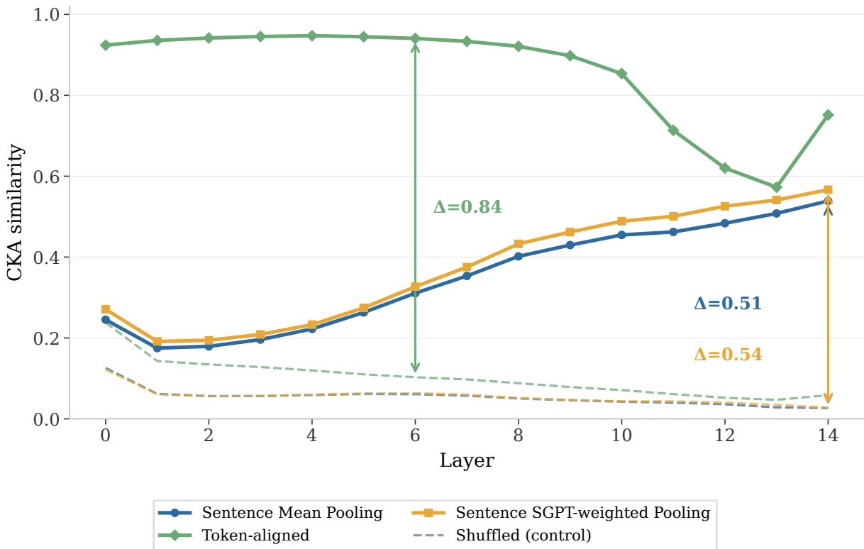
Layerwise CKA — B1 balanced
