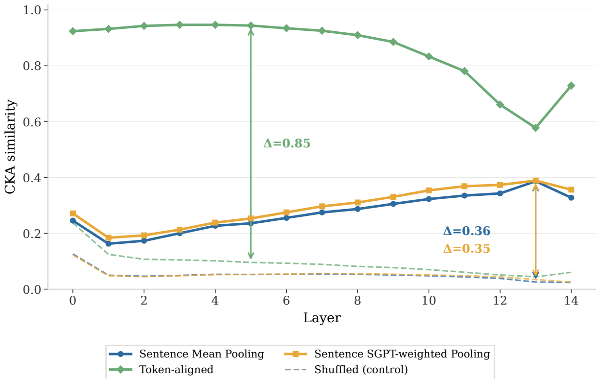
Layerwise CKA — B3 sequential
