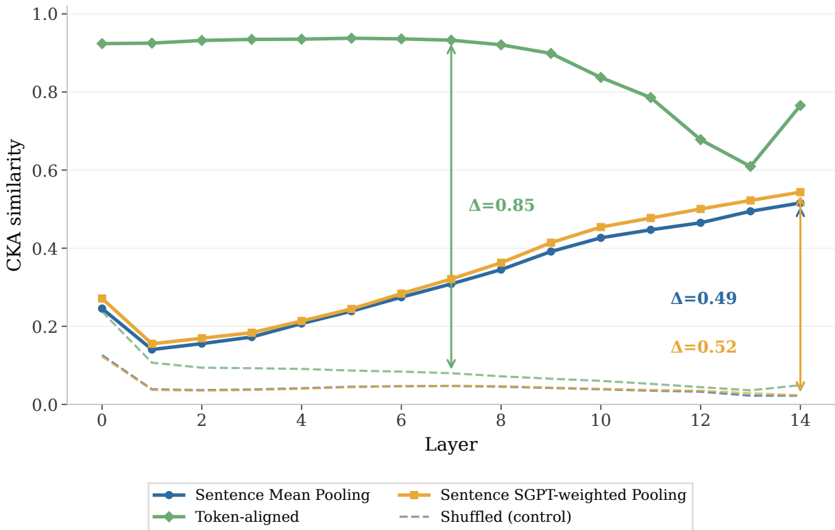
Layerwise CKA — B4 classroom
