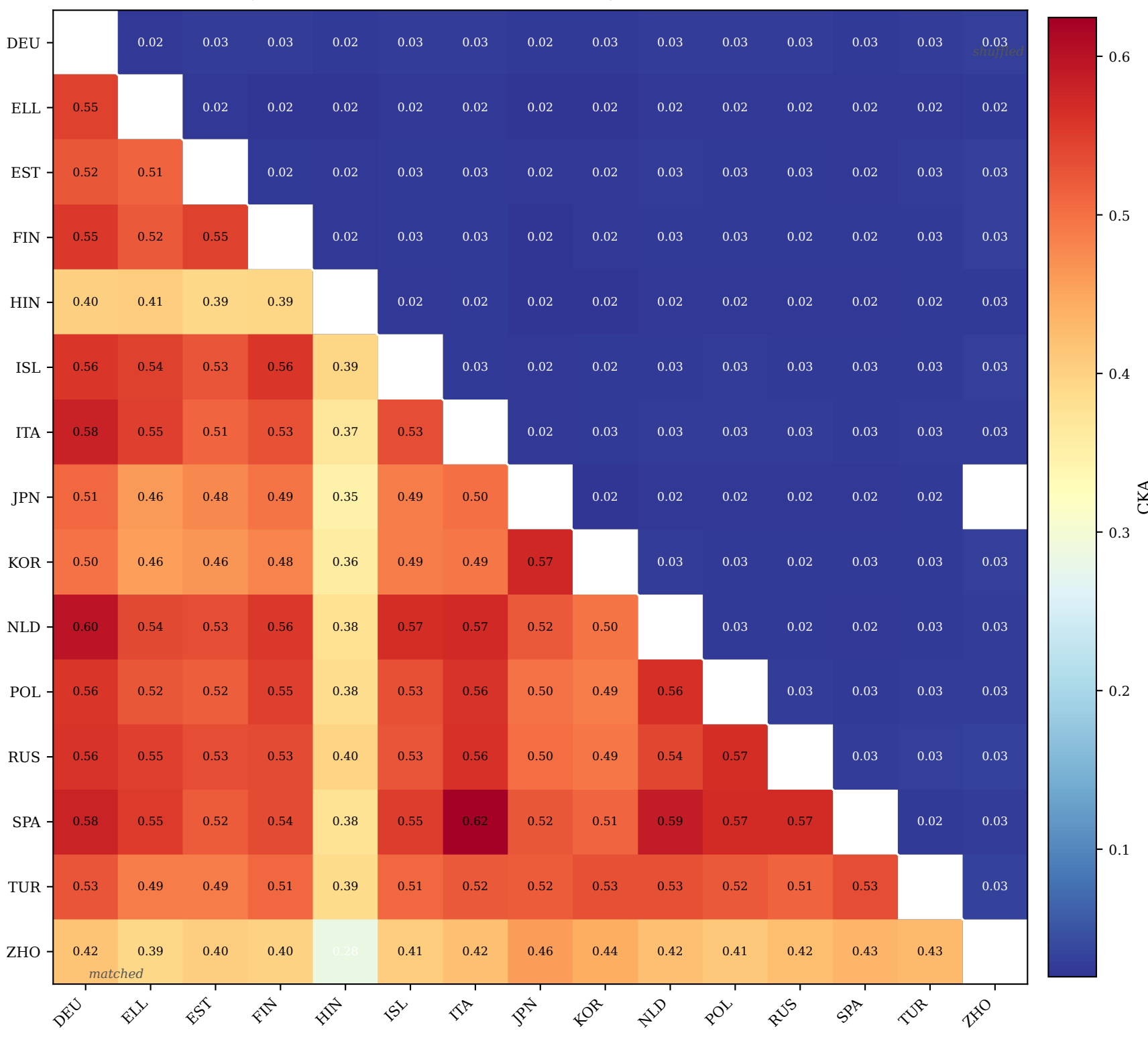
Last-layer pairwise CKA (Beetle monolingual, FineWeb-100M, SGPT)
