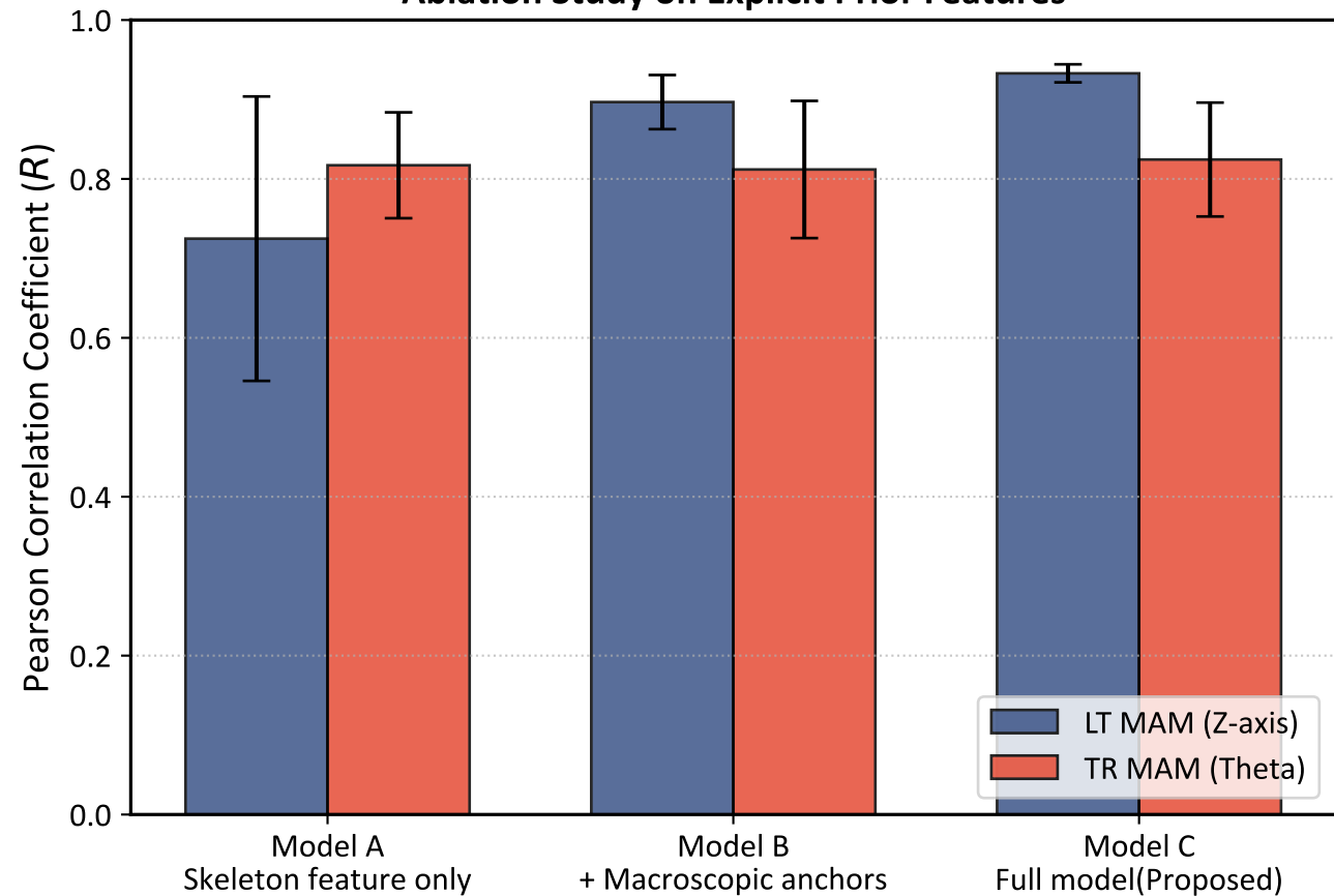
Ablation Study on Explicit Prior Features
